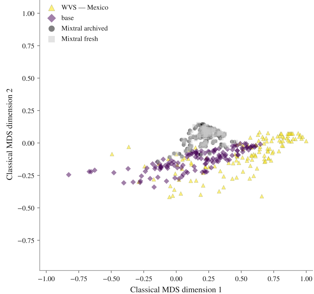
FA · 131 subpopulations · mean nEMD base 0.130, Mixtral archived 0.109, Mixtral fresh 0.125
