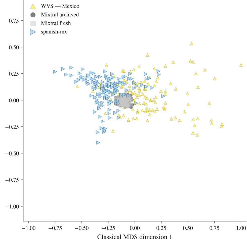
FA · 130 subpopulations · mean nEMD Mixtral archived 0.132, Mixtral fresh 0.148, spanish-mx 0.140
