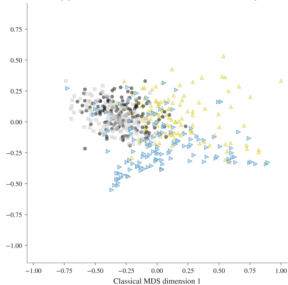
FA · 130 subpopulations · mean nEMD Mixtral archived 0.132, Mixtral fresh 0.148, spanish-mx 0.140
