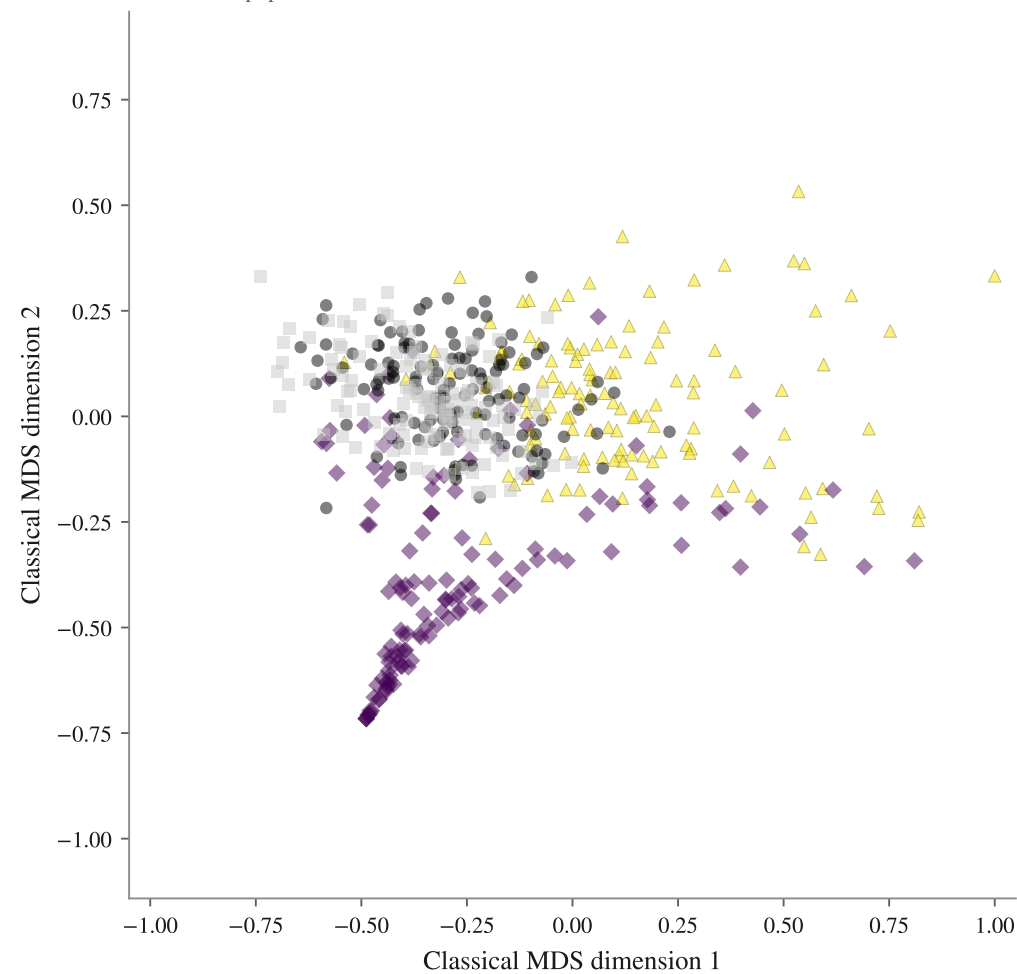
FA · 130 subpopulations · mean nEMD base 0.182, Mixtral archived 0.132, Mixtral fresh 0.148
