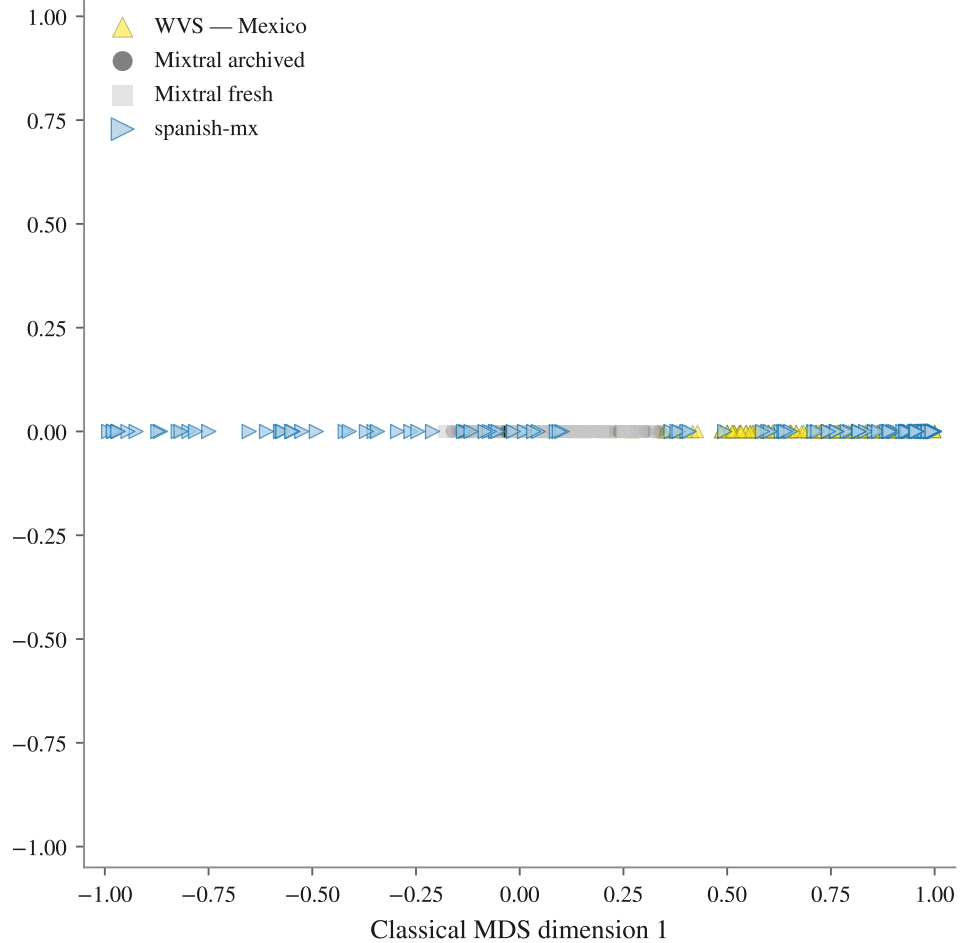
NTP · 130 subpopulations · mean nEMD Mixtral archived 0.276, Mixtral fresh 0.277, spanish-mx 0.279
