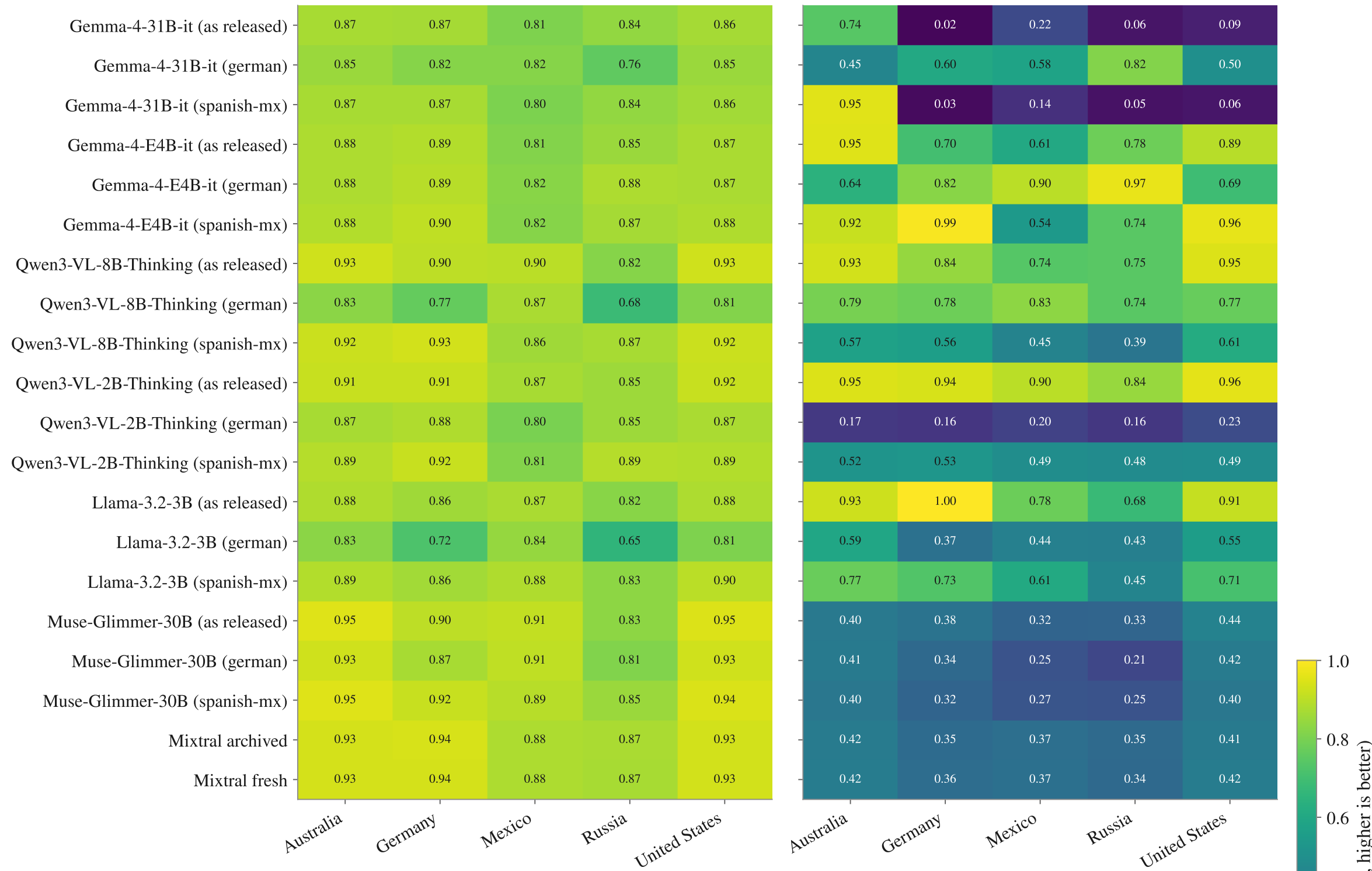
Accuracy: 1 - mean nEMD
