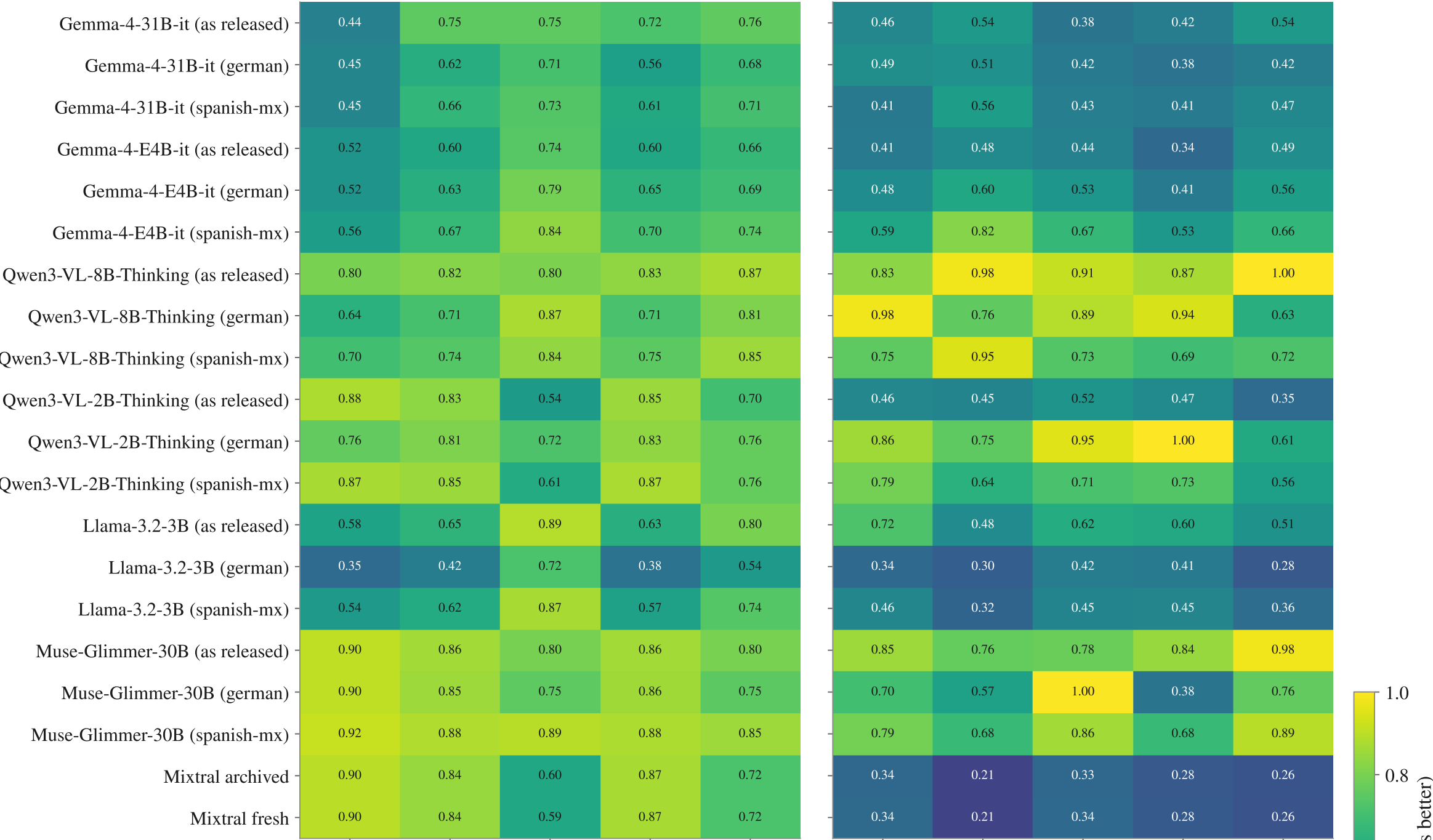
Accuracy: 1 - mean nEMD
