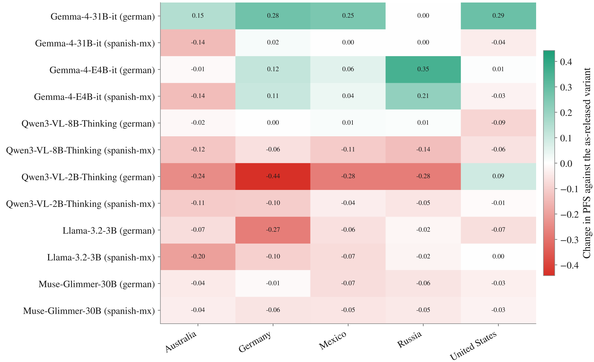
Finetuning change in fidelity — Country, happiness, NTP
