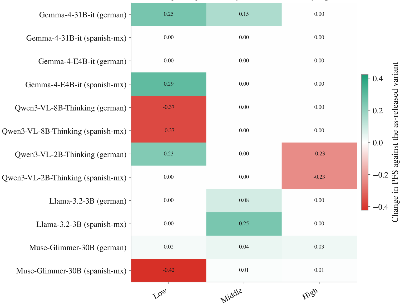
Finetuning change in fidelity — Education, every topic, FA
