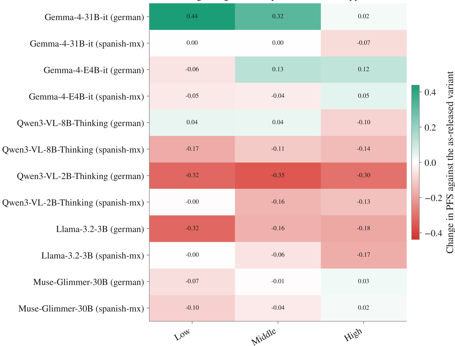
Finetuning change in fidelity — Education, happiness, FA
