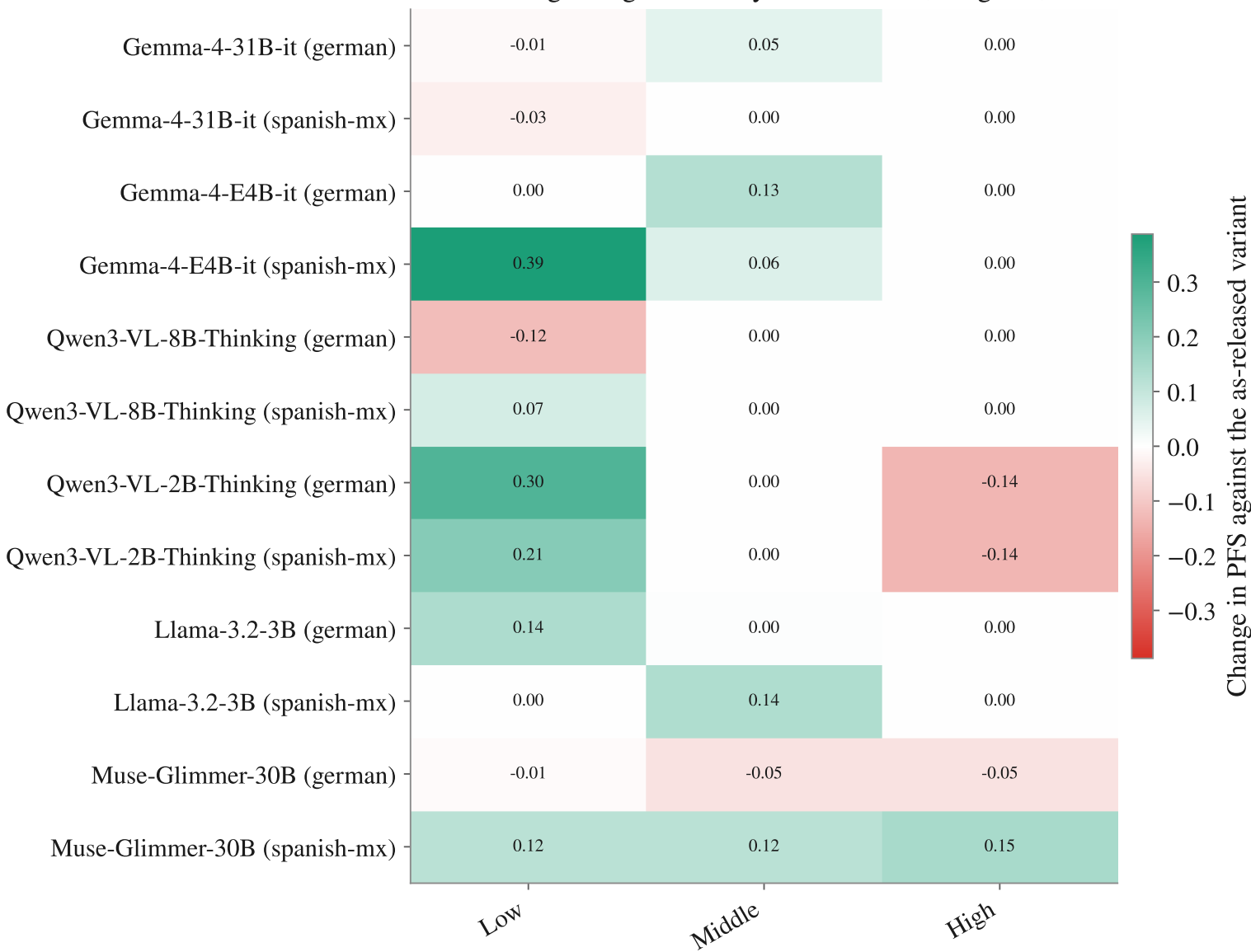
Finetuning change in fidelity — Education, religious, FA
