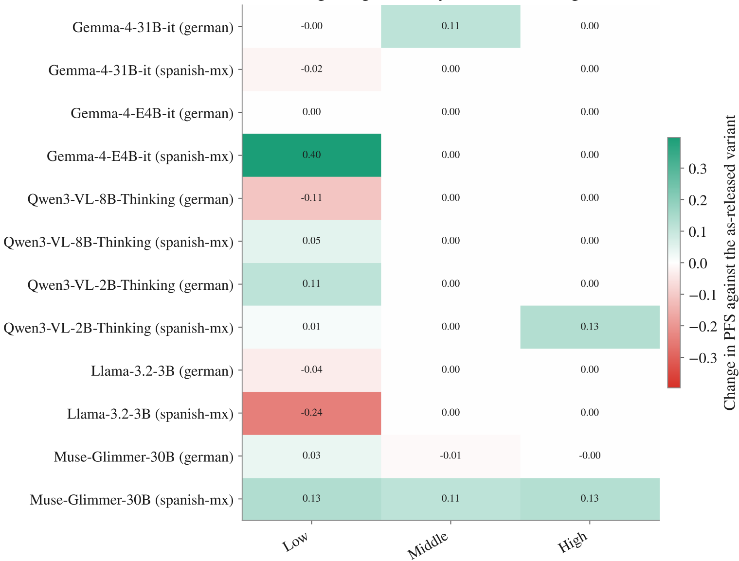
Finetuning change in fidelity — Education, religious, NTP
