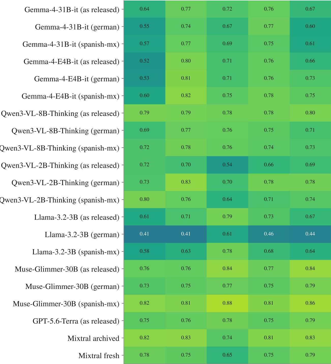
Accuracy: 1 - mean nEMD
