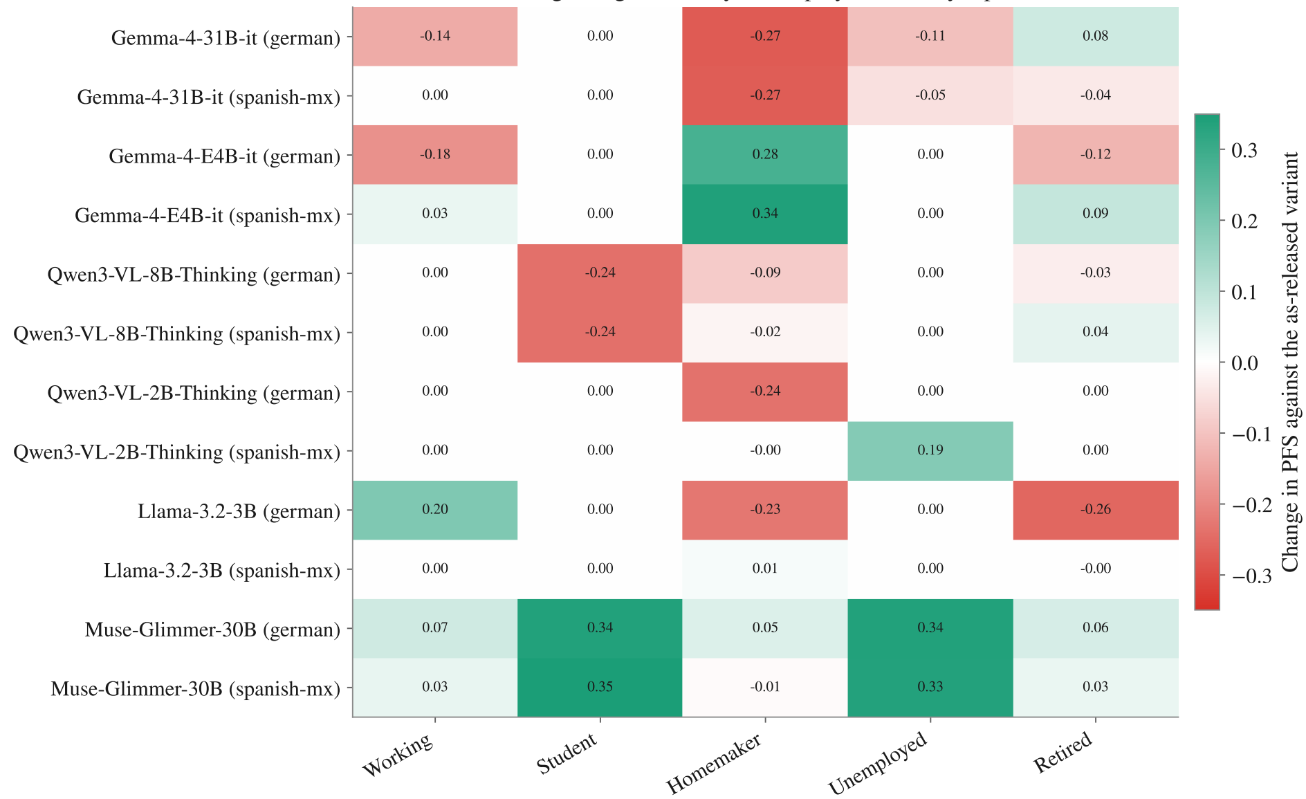
Finetuning change in fidelity — Employment, every topic, NTP
