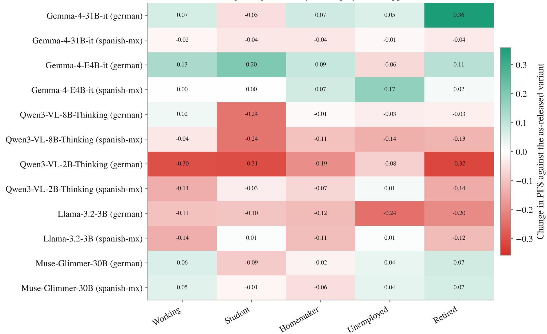
Finetuning change in fidelity — Employment, happiness, NTP
