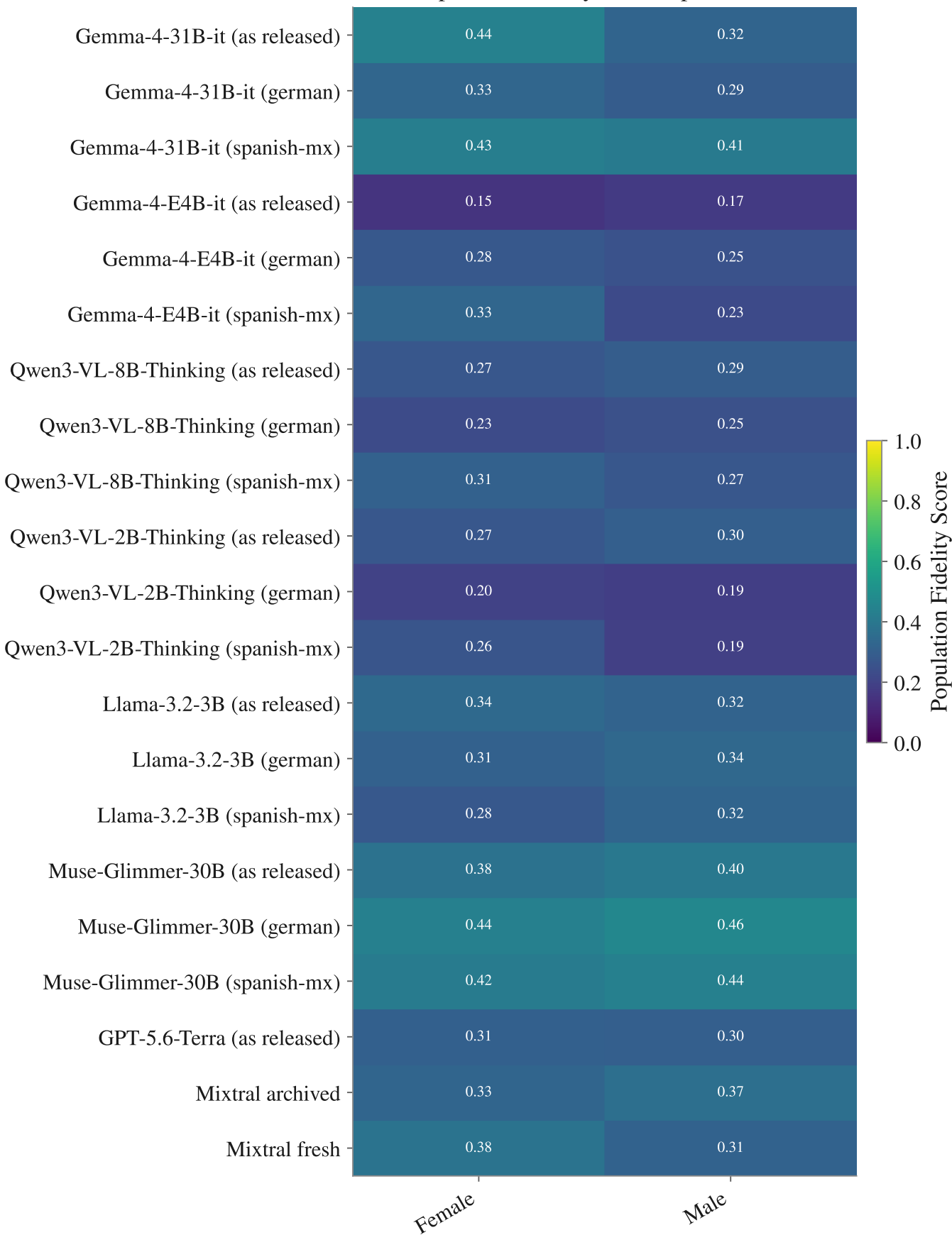
Population fidelity — Sex, politics, FA
