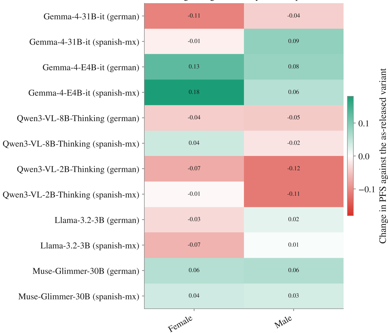
Finetuning change in fidelity — Sex, politics, FA
