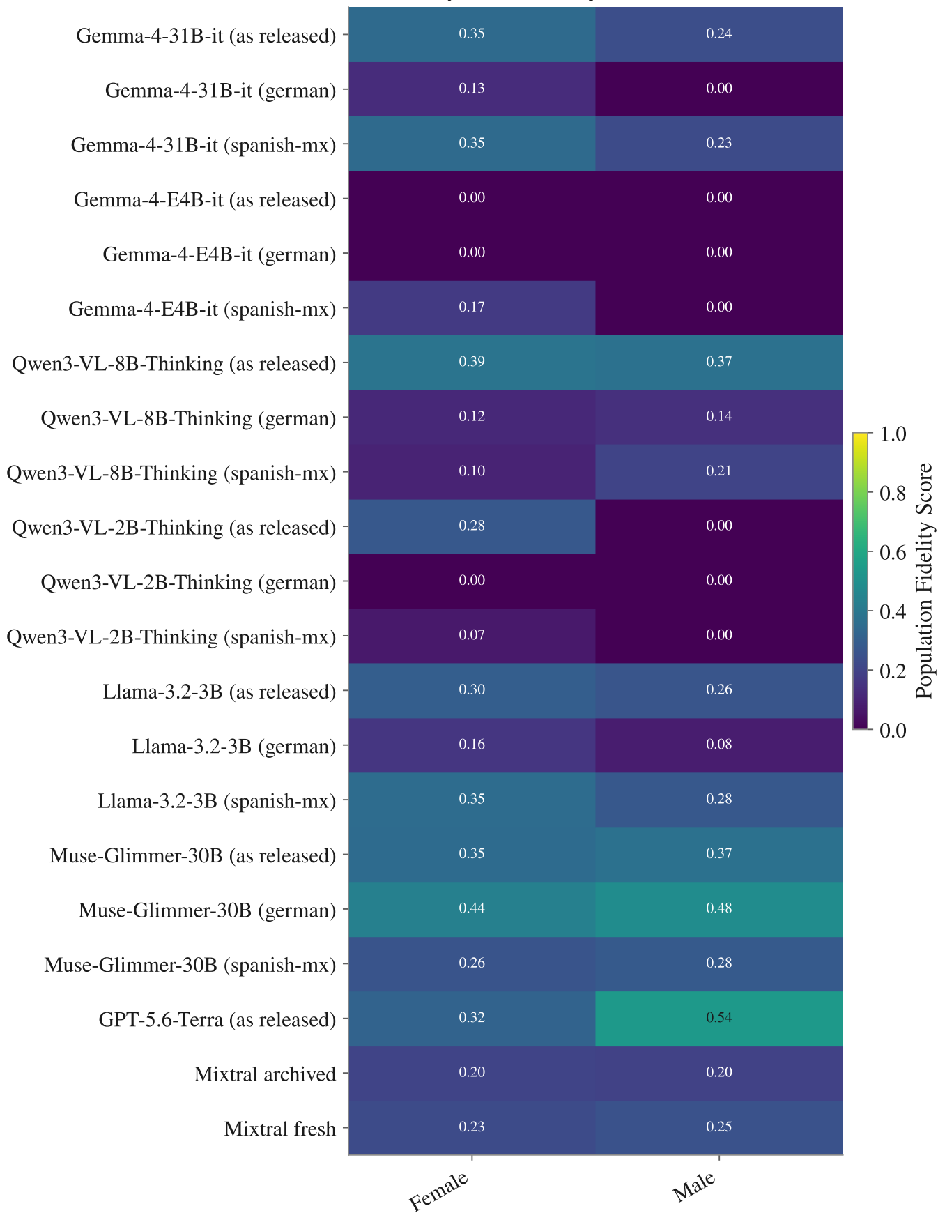
Population fidelity — Sex, trust, FA
