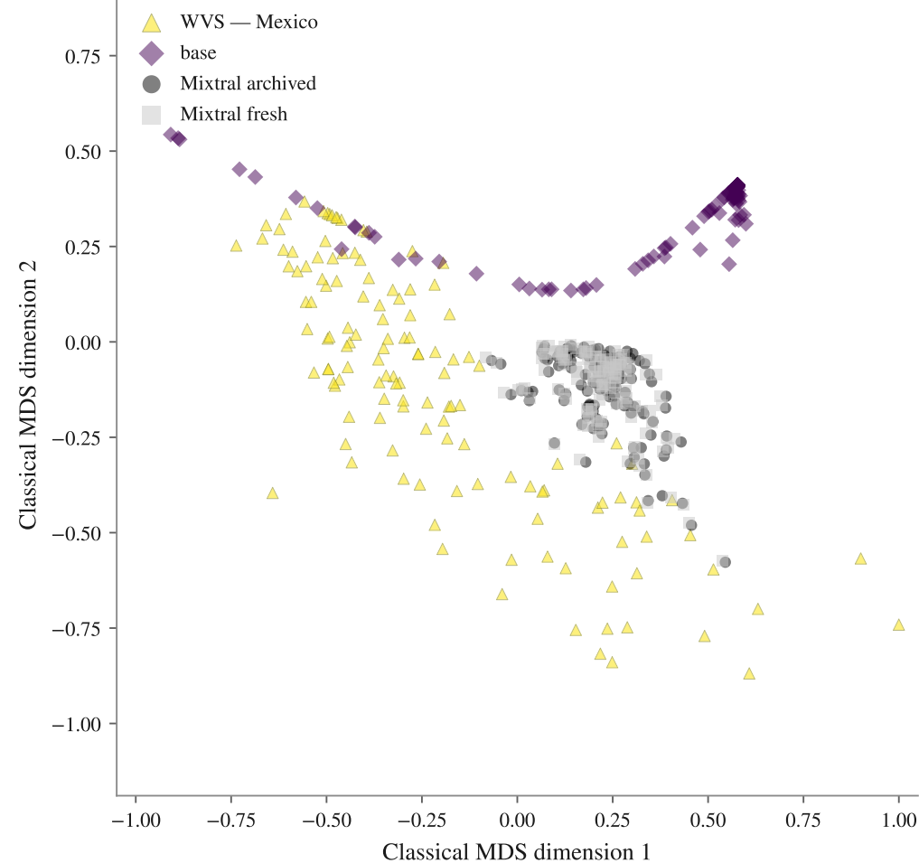
FA · 131 subpopulations · mean nEMD base 0.195, Mixtral archived 0.109, Mixtral fresh 0.125
