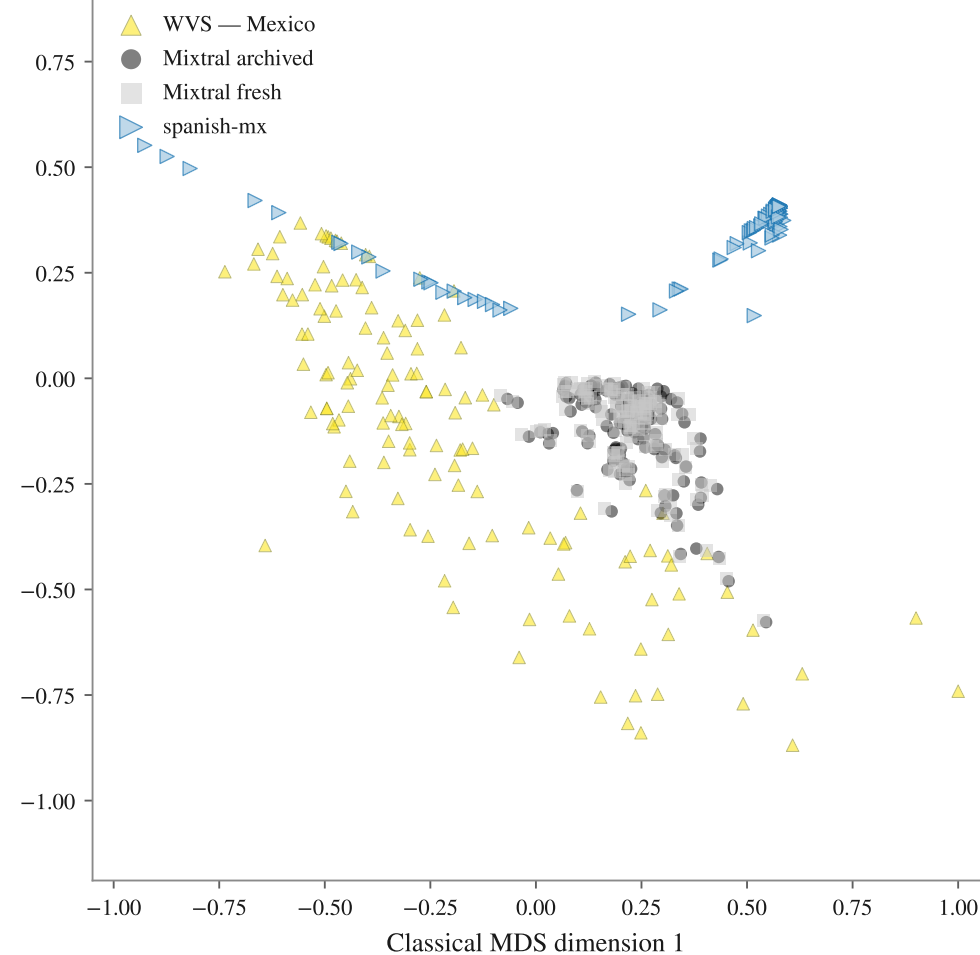
FA · 131 subpopulations · mean nEMD Mixtral archived 0.109, Mixtral fresh 0.125, spanish-mx 0.200
