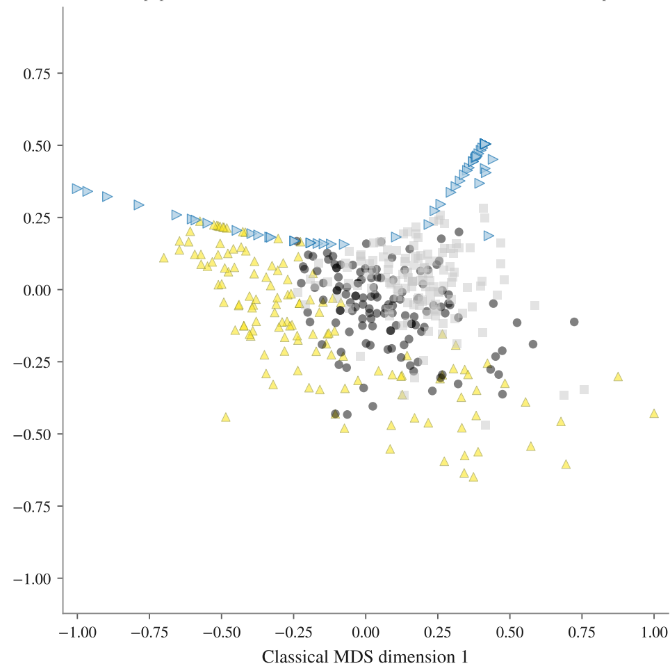
FA · 131 subpopulations · mean nEMD Mixtral archived 0.109, Mixtral fresh 0.125, spanish-mx 0.200
