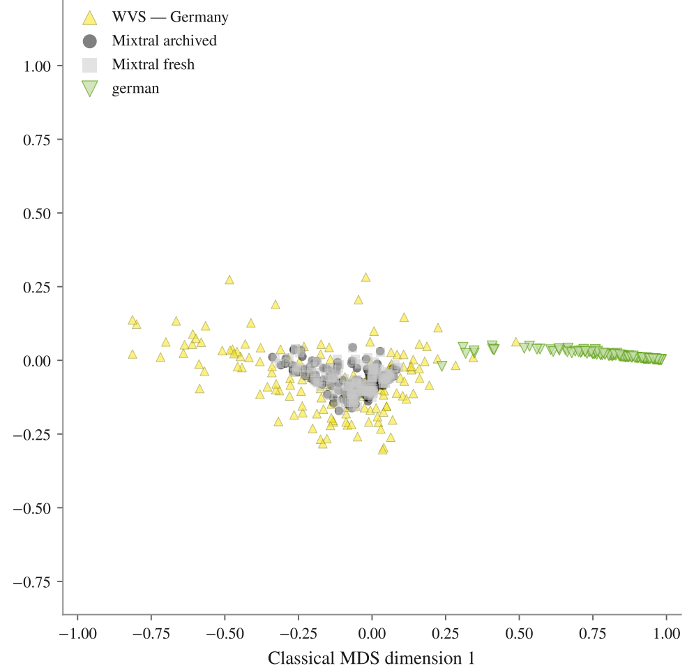
FA · 144 subpopulations · mean nEMD Mixtral archived 0.092, Mixtral fresh 0.074, german 0.295
