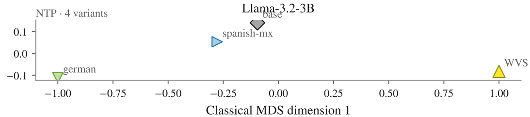
Classical MDS dimension 2
