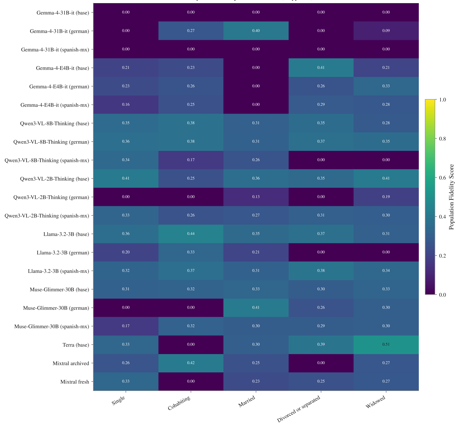
Population fidelity — Marital status, happiness, FA
