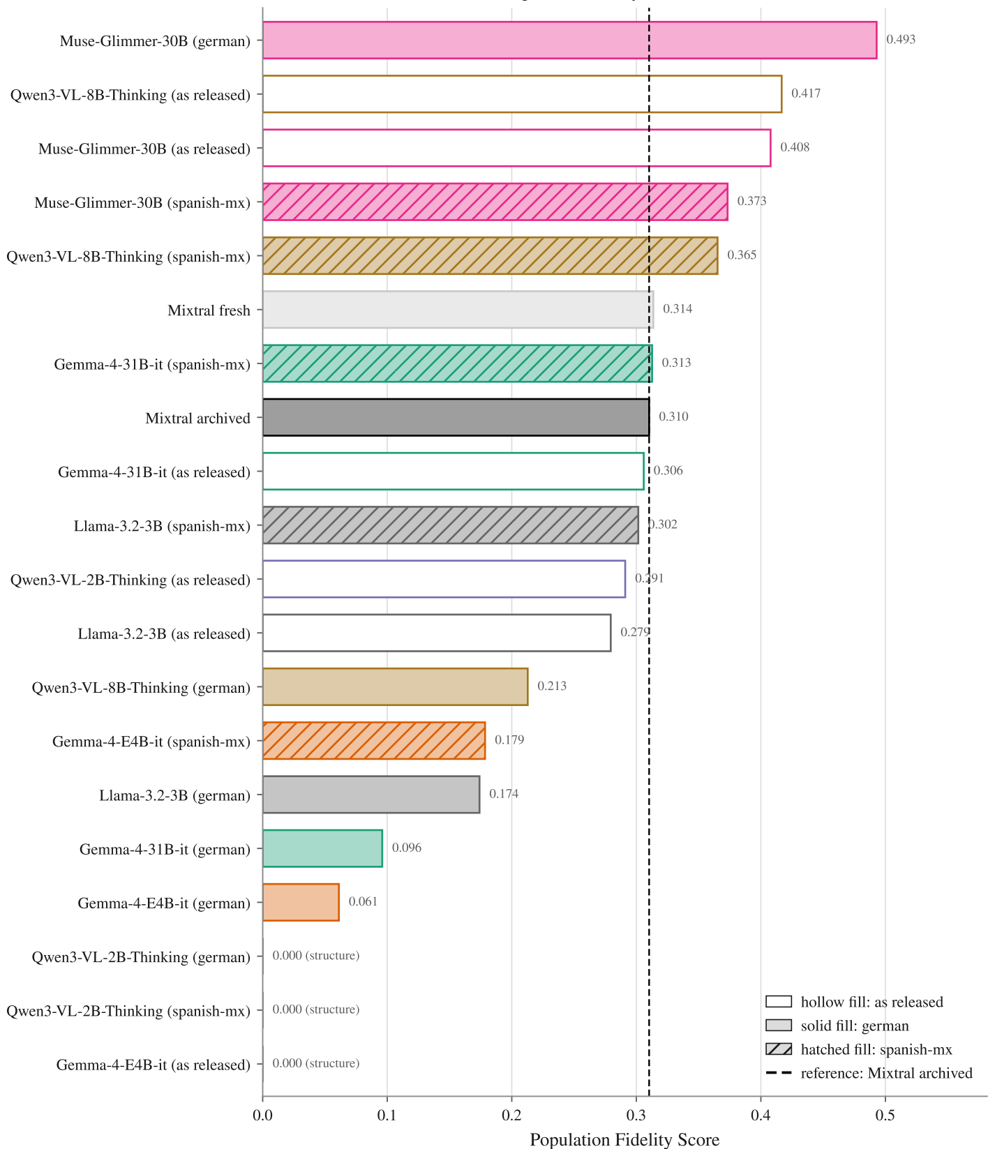
Population fidelity — trust, NTP
