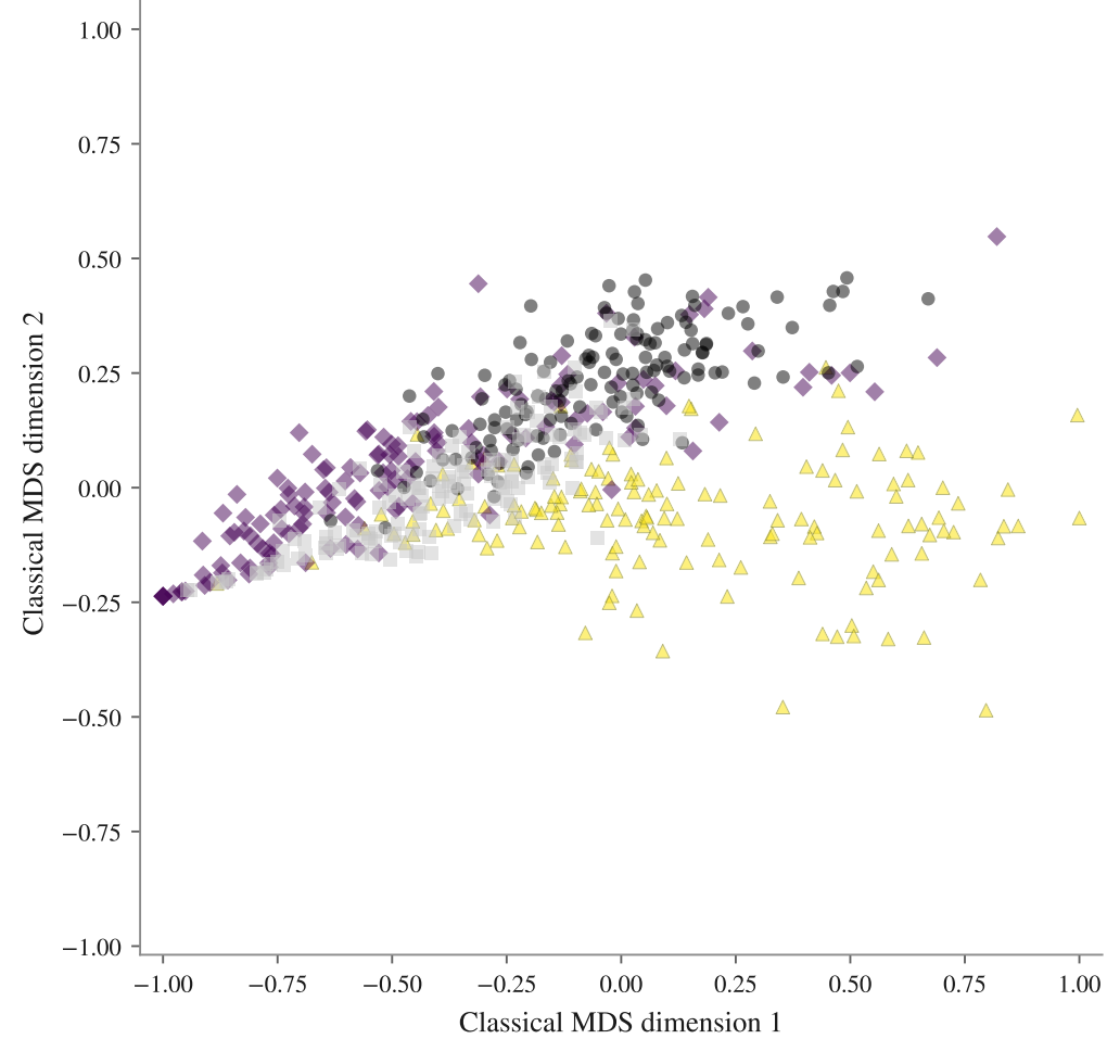
FA · 144 subpopulations · mean nEMD base 0.192, Mixtral archived 0.156, Mixtral fresh 0.176
