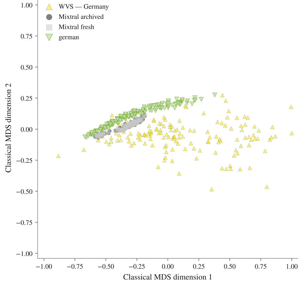
NTP · 144 subpopulations · mean nEMD Mixtral archived 0.155, Mixtral fresh 0.156, german 0.147
