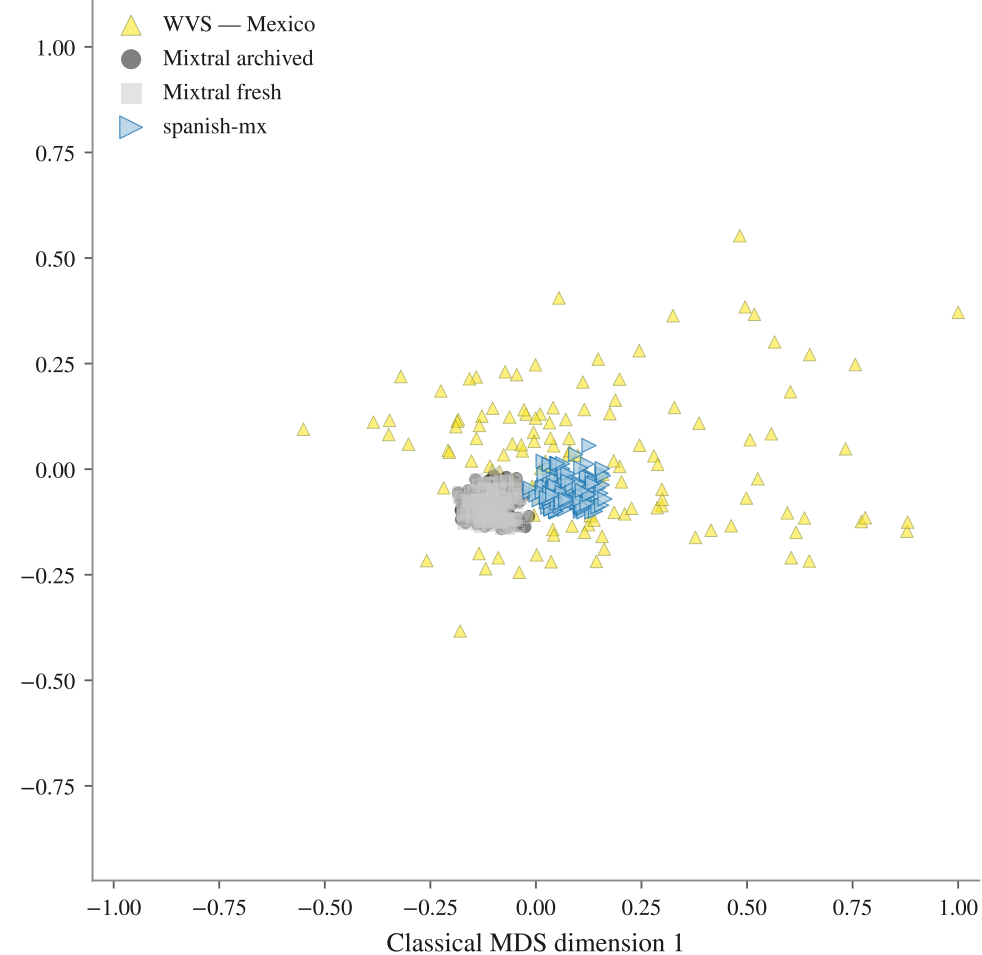
FA · 131 subpopulations · mean nEMD Mixtral archived 0.132, Mixtral fresh 0.149, spanish-mx 0.115
