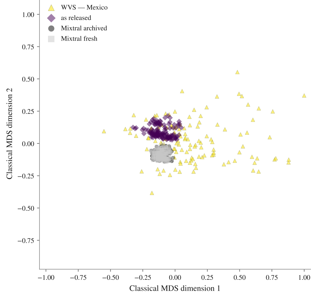
FA · 131 subpopulations · mean nEMD base 0.168, Mixtral archived 0.132, Mixtral fresh 0.149
