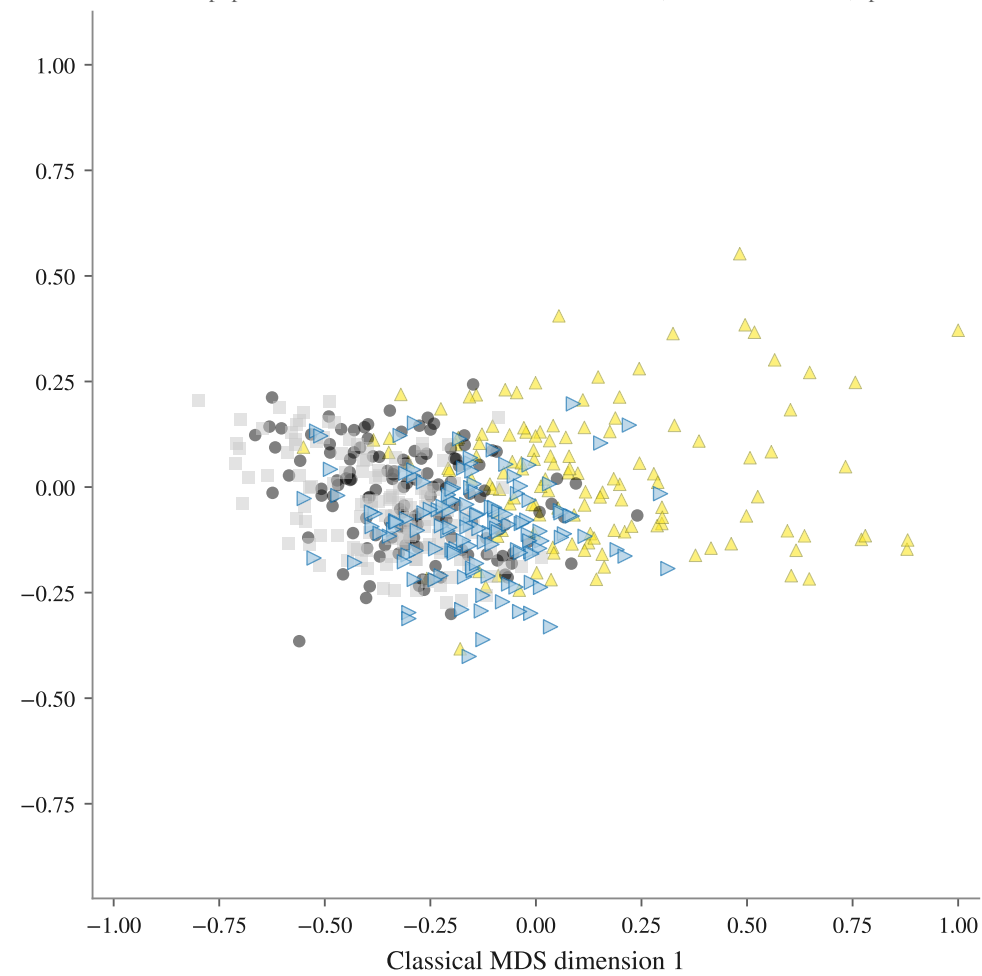
FA · 131 subpopulations · mean nEMD Mixtral archived 0.132, Mixtral fresh 0.149, spanish-mx 0.115
