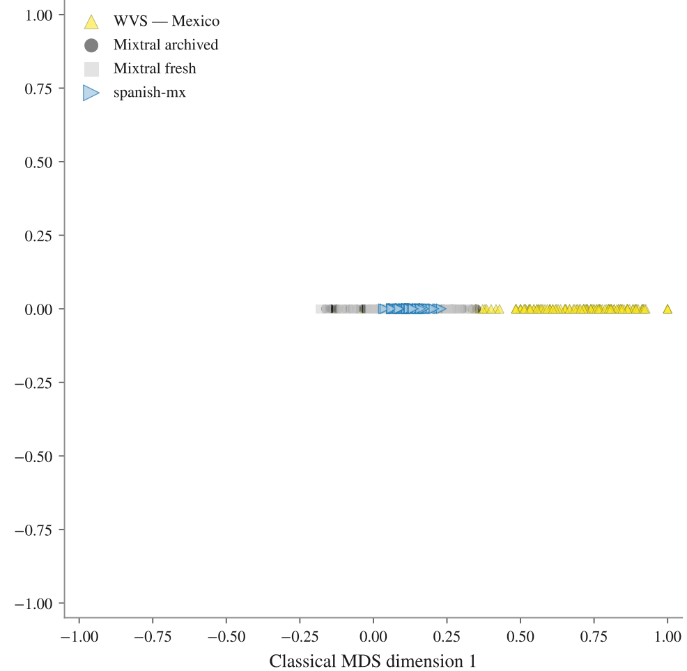
FA · 131 subpopulations · mean nEMD Mixtral archived 0.442, Mixtral fresh 0.282, spanish-mx 0.390
