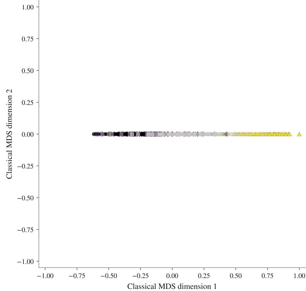
FA · 131 subpopulations · mean nEMD base 0.423, Mixtral archived 0.442, Mixtral fresh 0.282
