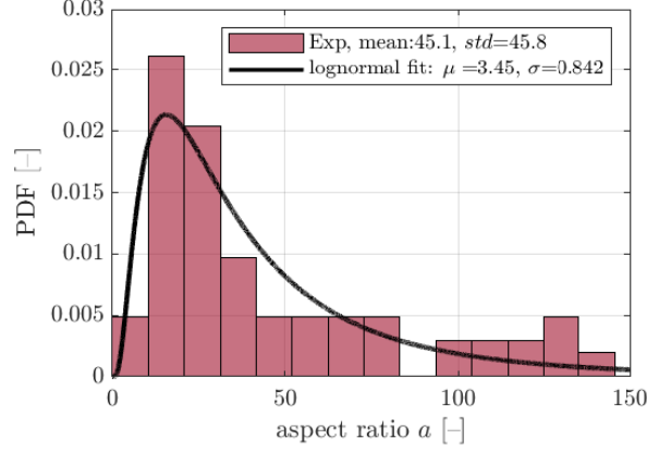
Figure B.11: Experimentally measured histogram for aspect ratios of flax fibers from [?] and lognormal fit according to (??)
