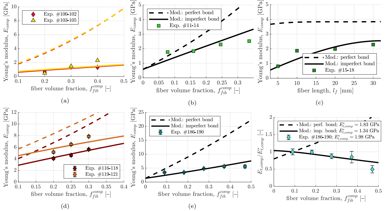
Figure 5: Validation of composite for imperfect bond: Longitudinal (a-e) and transversal (f) Young's modulus tested by (a) ? ] for HDPE-hemp [Exp.#100-105, \bar{\alpha} = \bar{\beta} = 37.3/\text{MPa} ], (b-c) ? ] for polyester-pineapple leaf fiber (PALF) [Exp.#11-18, \bar{\alpha} = \bar{\beta} = 1870/\text{MPa} ], (d) ? ] for PP-flax [Exp.#116-118, \bar{\alpha} = \bar{\beta} = 5.3 \text{ m}/\text{MPa} ] and PLA-flax [Exp.#117-119, \bar{\alpha} = \bar{\beta} = 4.3/\text{MPa} ], and (e-f) ? ] for polyester-jute [Exp.#186-190, \bar{\alpha} = \bar{\beta} = 2680/\text{MPa} ] as function of the fiber volume fraction (a-b,d-f) and fiber length (c); imperfect bond model (continuous lines) with fitted interface compliances \bar{\alpha} = \bar{\beta} compared to perfect bond predictions (dashed lines)
