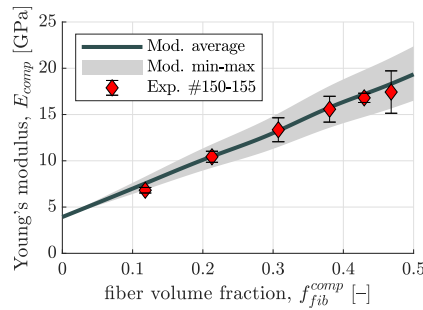
Figure 4: Longitudinal Young's modulus for perfectly bonded Phormium-epoxy composites tested by ? ] as a function of the fiber volume fraction using a representative average of physical fiber properties (central thick line) and minimum/maximum fiber properties (gray area)
