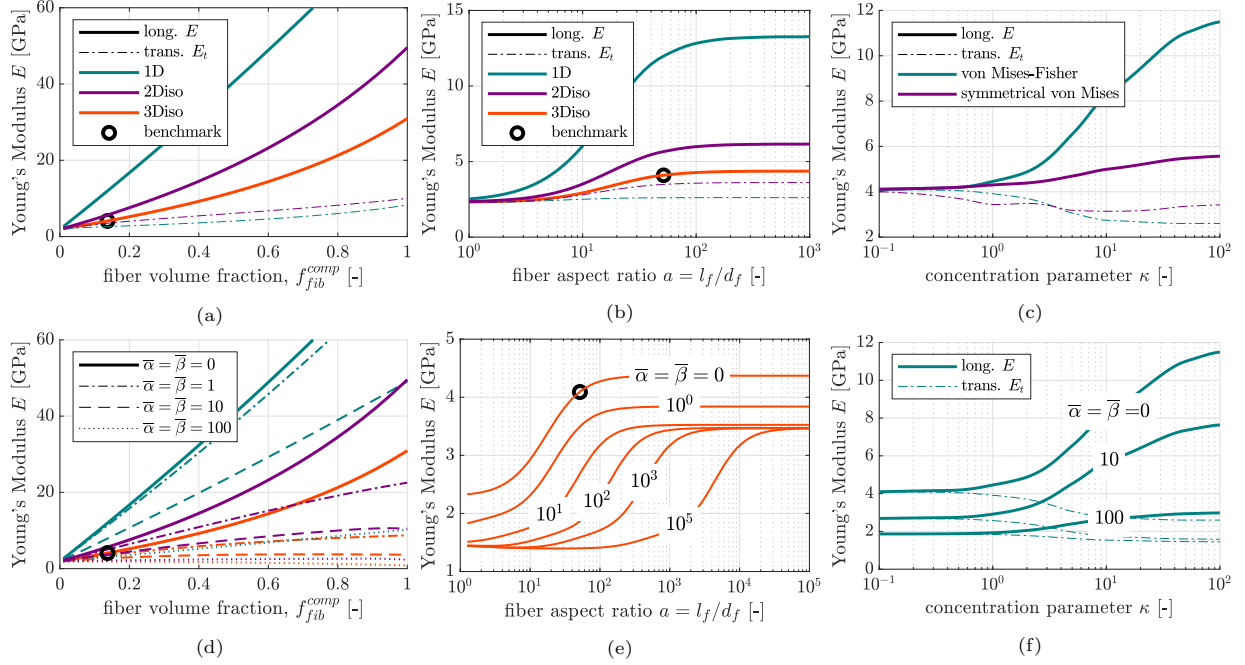
Figure 6: Sensitivity analyses of the composite's Young's modulus ( E ... in plane or longitudinal modulus and E_t ... transversal modulus) based on benchmark composition for perfectly bonded fibers (top row) and imperfectly bonded fibers (with interface compliance \bar{\alpha} = \bar{\beta} with unit [1/GPa], bottom row) and with different fiber orientations (1D ... aligned, 2Diso ... isotropically oriented in a plane, 3Diso ... isotropic in all directions): (a)+(d) w.r.t fiber volume fraction (b)+(e) w.r.t. the fiber aspect ratio, (c)+(f) w.r.t. concentration parameter of von Mises Fisher and (symmetrical) von Mises distribution function; note that (e) is limited to 3Diso orientations and (f) to von Mises-Fisher distribution; black circle refers to the benchmark composition
