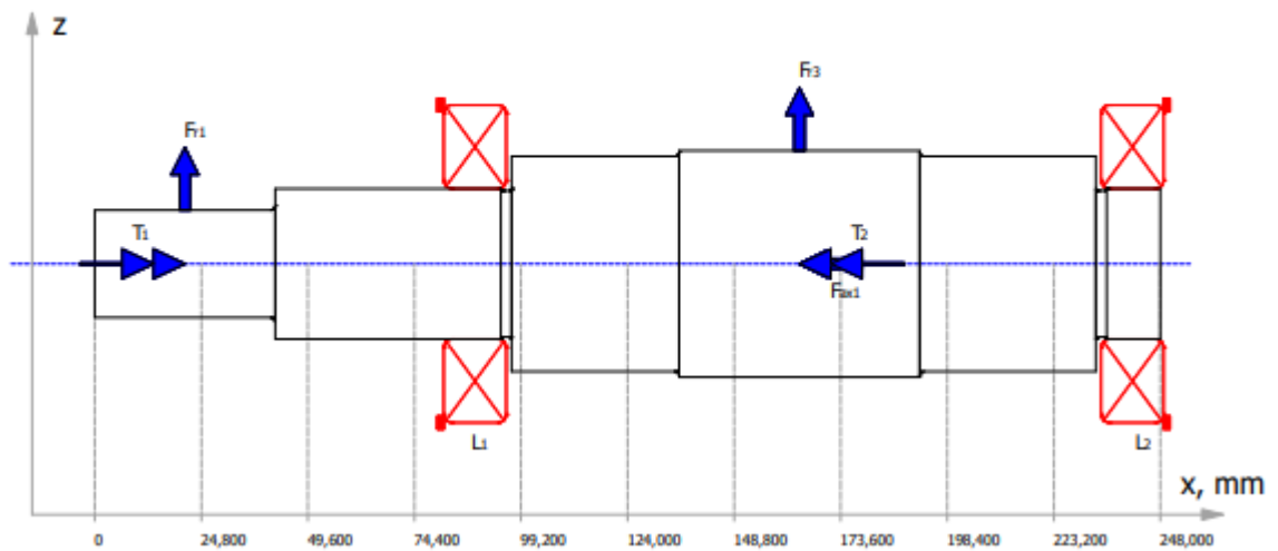
Calculation graphic Z-X-plane
