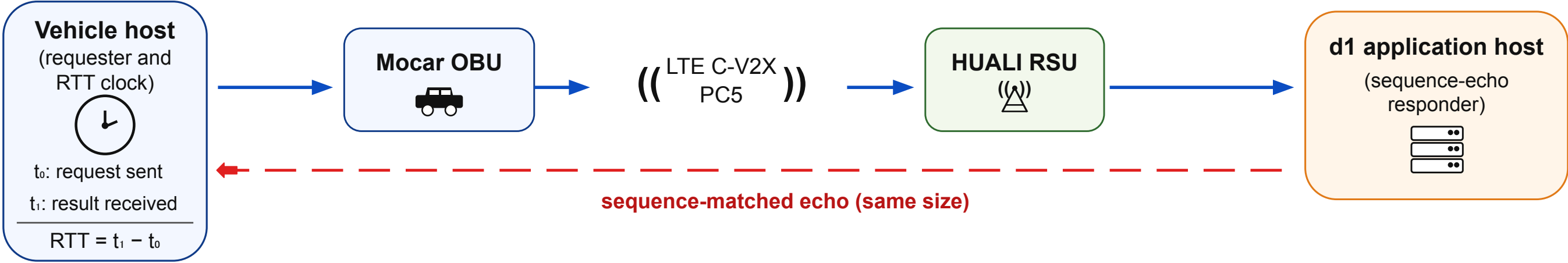
(a) Direct PC5 path
