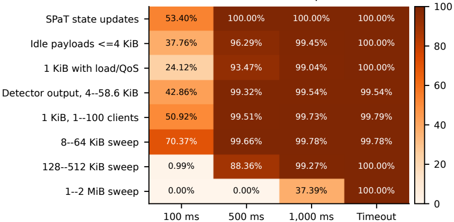
(a) Requests completed by deadline (% of all issued requests)
