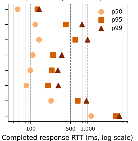
(b) Completed-response RTT percentiles
