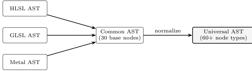
Fig. 3. Dual-AST architecture. Backend-specific ASTs preserve source language structure and extend a shared common AST. Normalization produces the universal AST used by all forward code generators.
