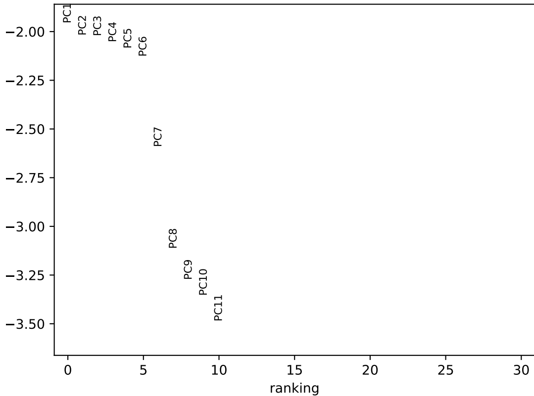
variance ratio
