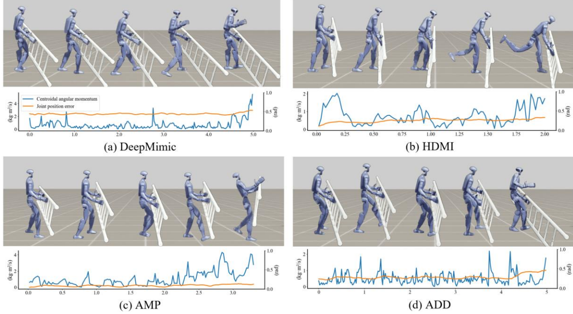
Fig 3: Qualitative results of ladder carry. Orange lines represent joint position tracking errors and blue lines show the payload-induced angular momentum (5 s before termination).
