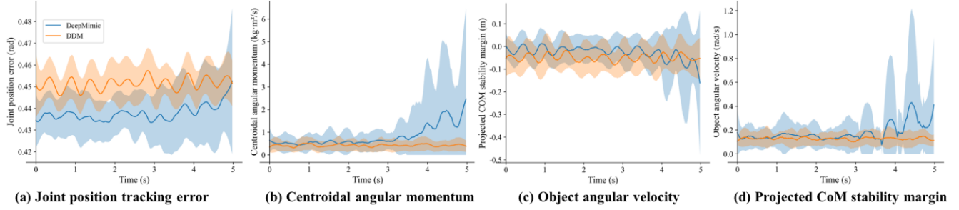
Fig 4: Effect of momentum-aware shaping on the ladder front-carry task. DDM is compared with DeepMimic. Shaded regions denote variation across trials.
