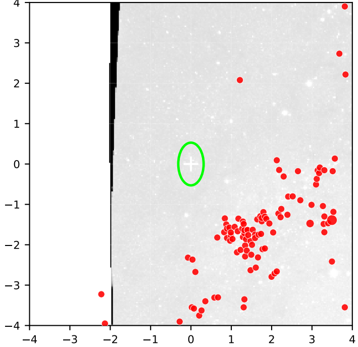
SITELLE SN3 Field2 deep coverage=75%
