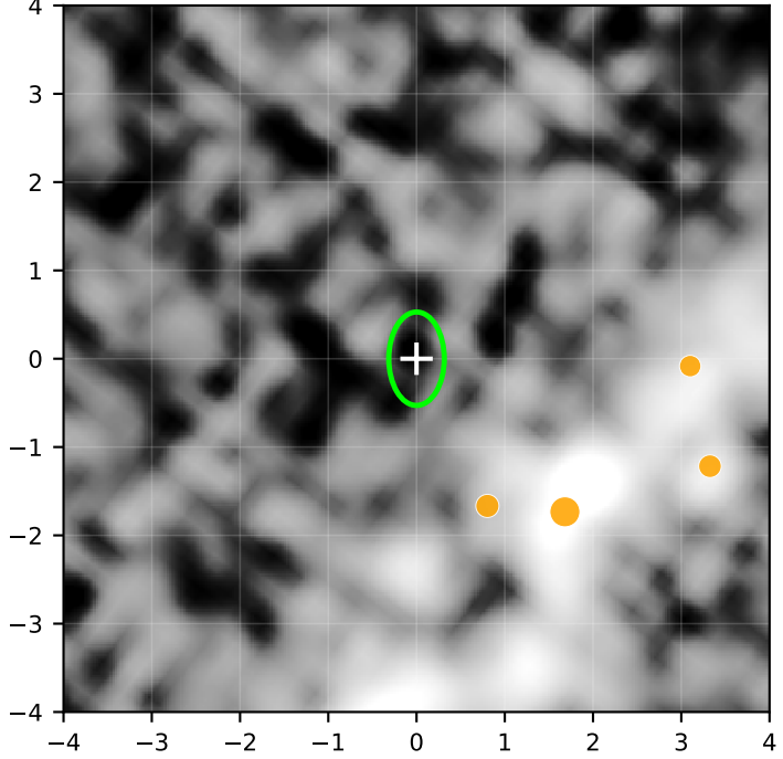
CO slab ok | ch=92-99 | Nchan=8
