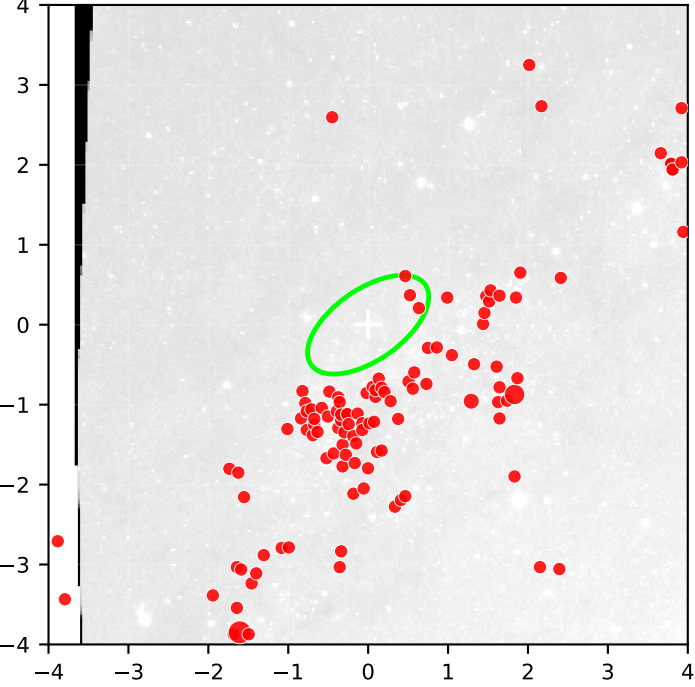
SITELLE SN3 Field2 deep coverage=96%
