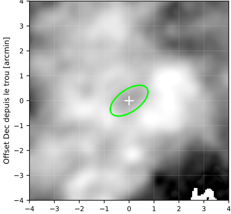
H I slab ch=67-69 | v=-229.3..-221.0 km/s | Nch=3
