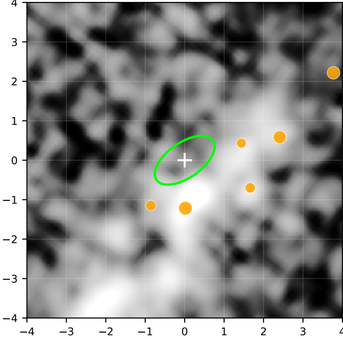
CO slab ok | ch=92-99 | Nchan=8
