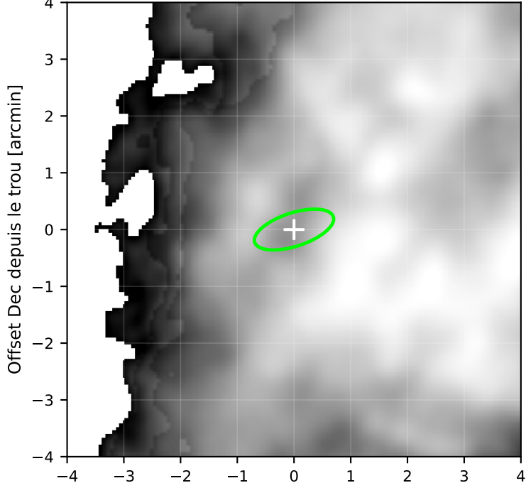
H I slab ch=63-65 | v=-212.8..-204.5 km/s | Nch=3
