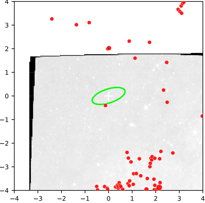
SITELLE SN3 Field2 deep coverage=66%
