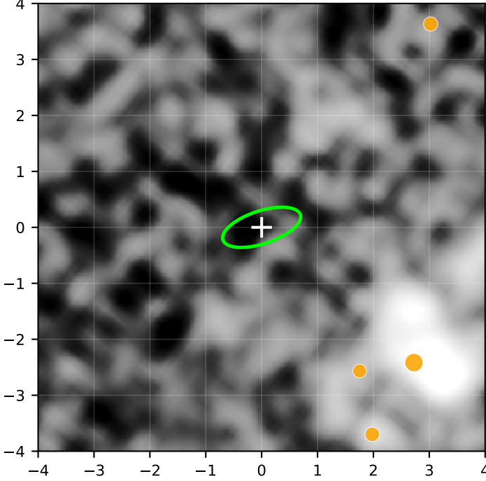
CO slab ok | ch=85-92 | Nchan=8
