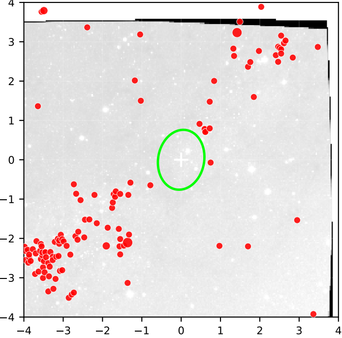
SITELLE SN3 Field2 deep coverage=92%
