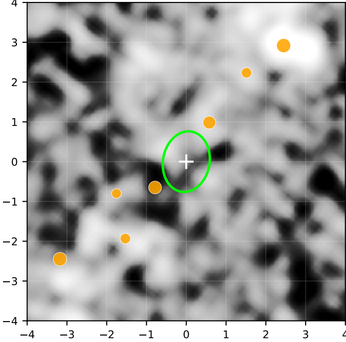
CO slab ok | ch=79-86 | Nchan=8
