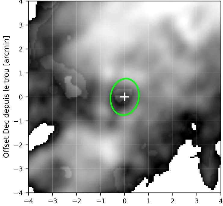
H I slab ch=59-61 | v=-196.3..-188.1 km/s | Nch=3
