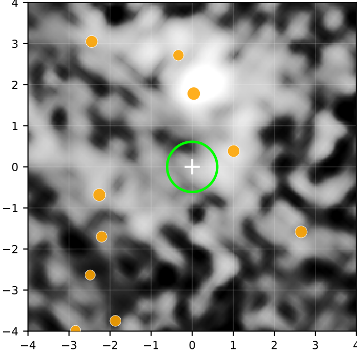
CO slab ok | ch=28-35 | Nchan=8
