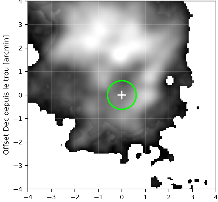
H I slab ch=27-29 | v=-64.3..-56.1 km/s | Nch=3
