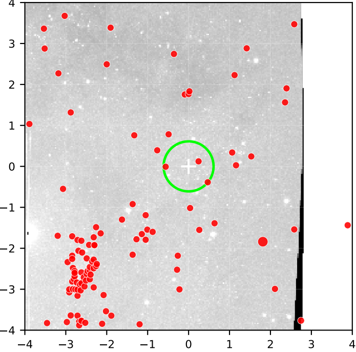
SITELLE SN3 Field1 deep coverage=85%
