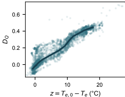
a Heating-capacity loss
