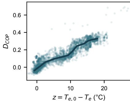
b COP loss
