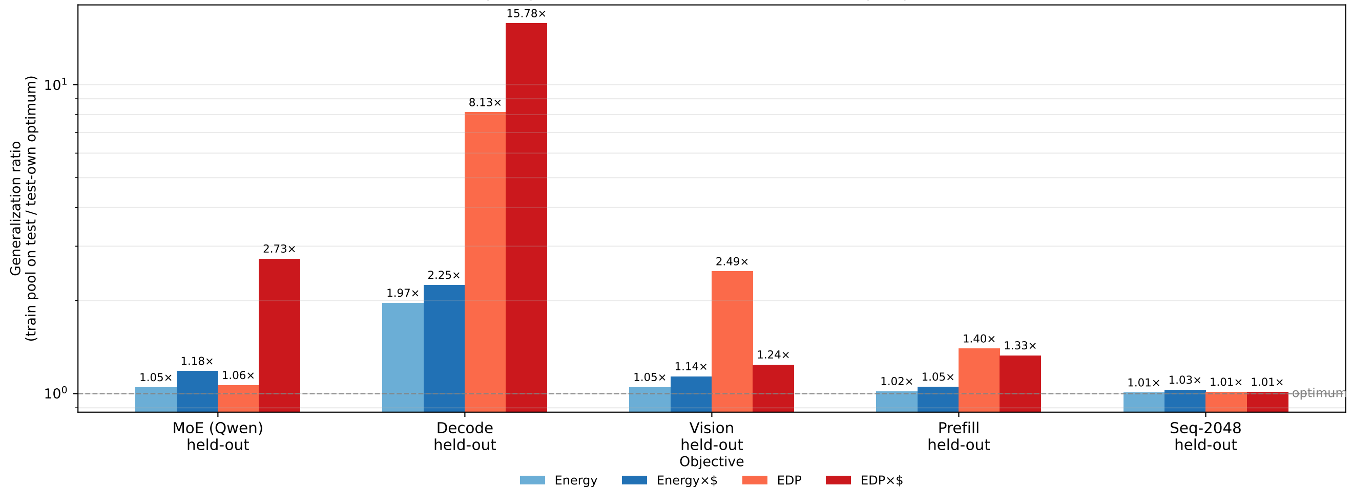
Train-pool generalization to held-out test sets (8-chiplet pools, v2)
