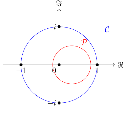
Figure 2: The two basepoint circles: the critical circle \mathcal{C} and the prime circle \mathcal{P} , with the axis intersections located by the five intersection theorems of Layer 3.
