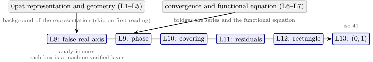
Figure 1: Structure of the development. The analytic core of the Riemann direction is the chain L8–L13 (boxed); the 0pat representation L1–L5 and the series/functional-equation layer L6–L7 are the background from which the core is assembled and may be skipped on a first reading. The odd/even pairing of iso 41 is machine-verified independently and closes Layer 13.
