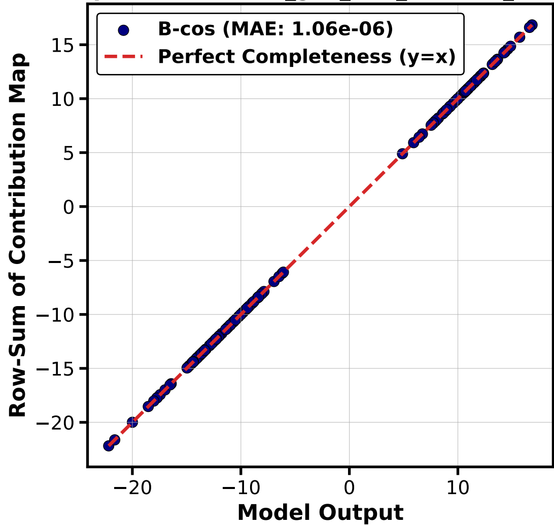
B-COS GCN Completeness (bcos_gcn_add_readout_then_agg, seed=0)
