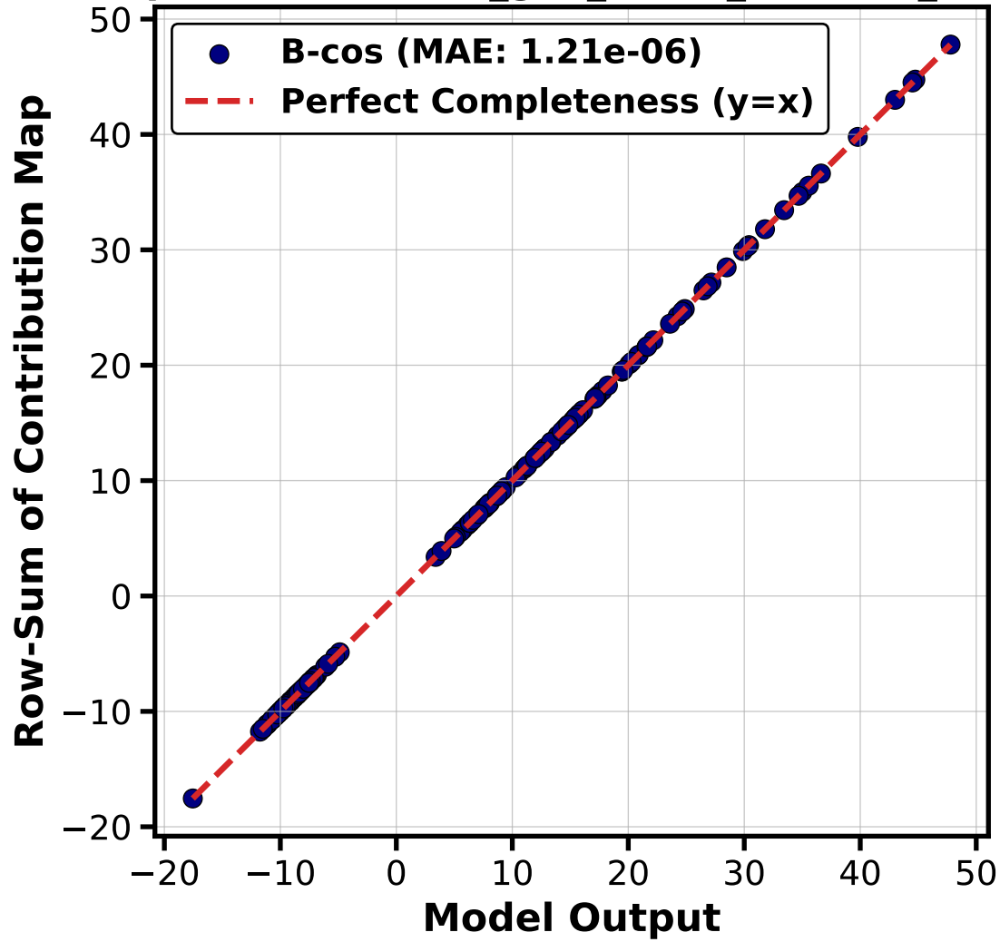
B-COS GCN Completeness (bcos_gcn_mean_readout_then_agg, seed=2)
