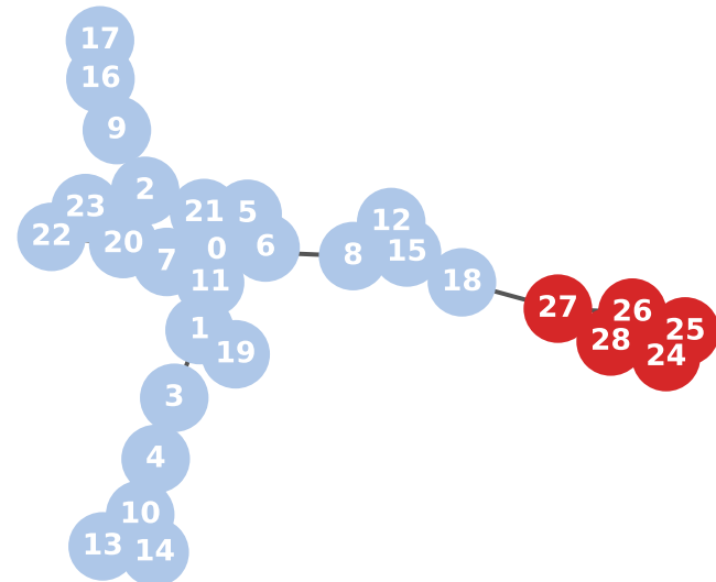
Jaccard Score: 0.67
