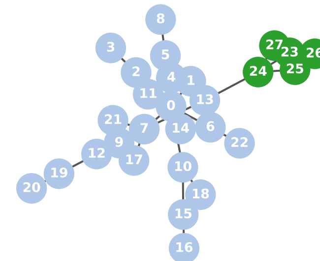
Jaccard Score: 1.00
