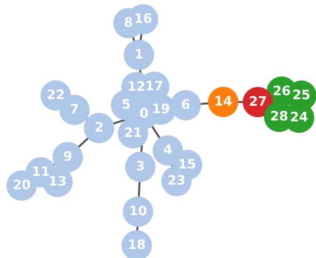
Jaccard Score: 0.67
