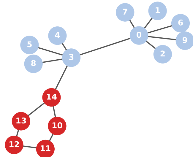
Jaccard Score: 1.00
