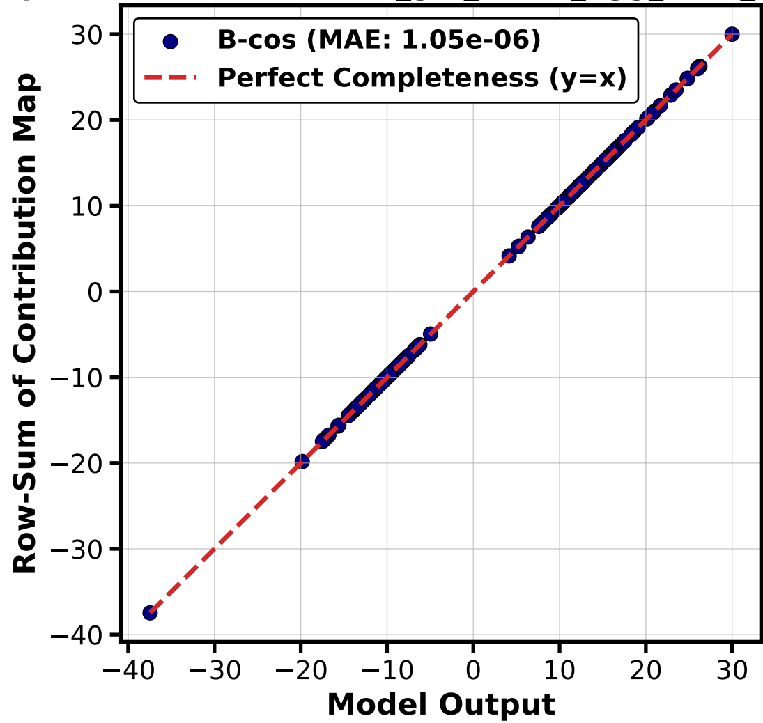
B-COS Completeness Check (bcos_gin_mean_agg_then_readout, seed=2)
