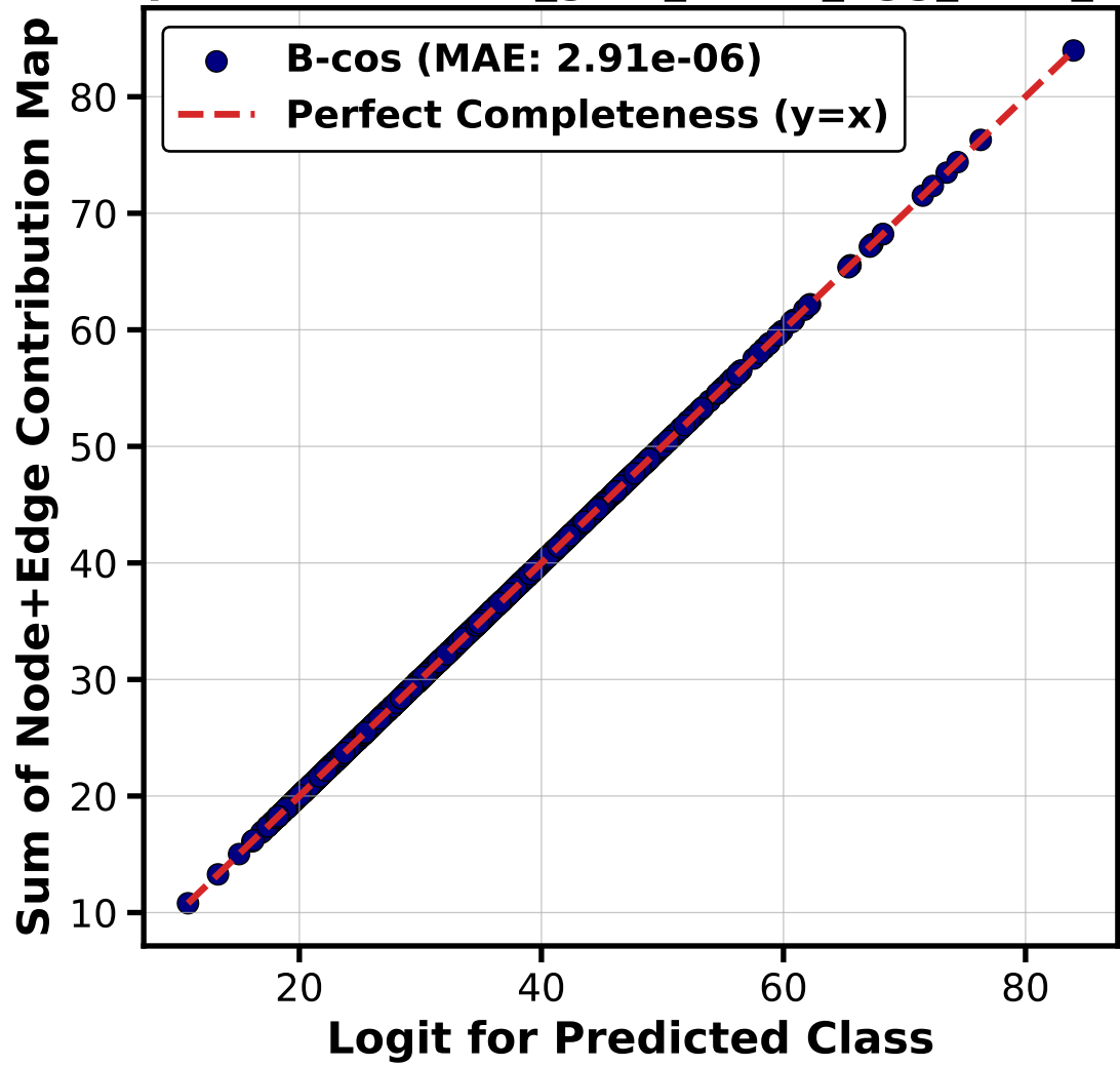
B-COS GINE Completeness (bcos_gine_mean_agg_then_readout, seed=0)
