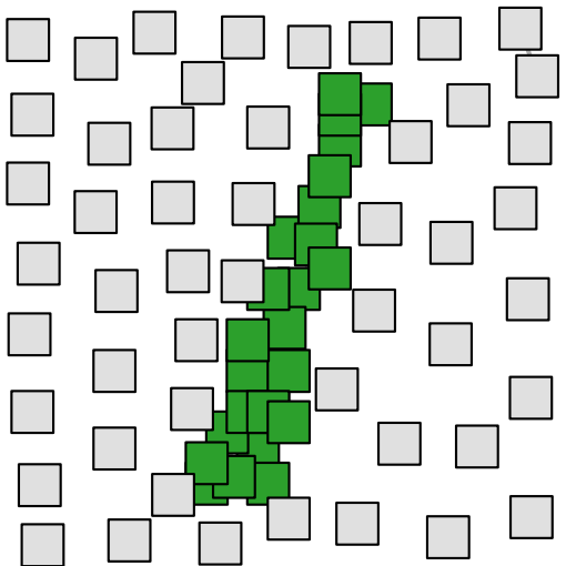
GT Label: 1
