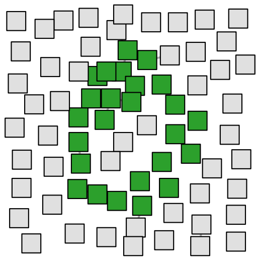
GT Label: 0
