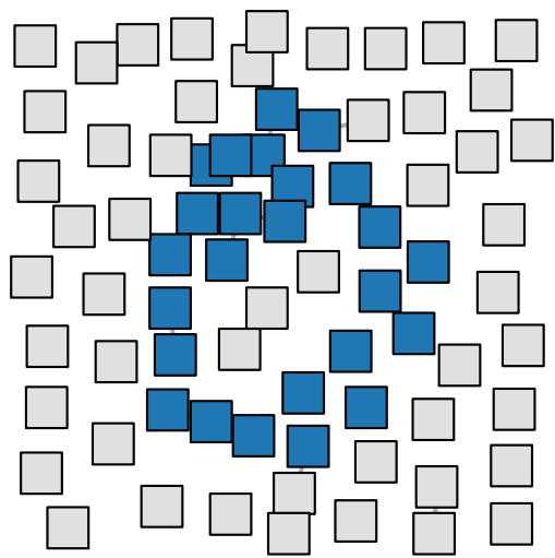
Predicted: 0
