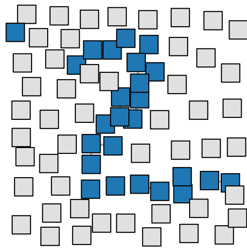
Predicted: 2
