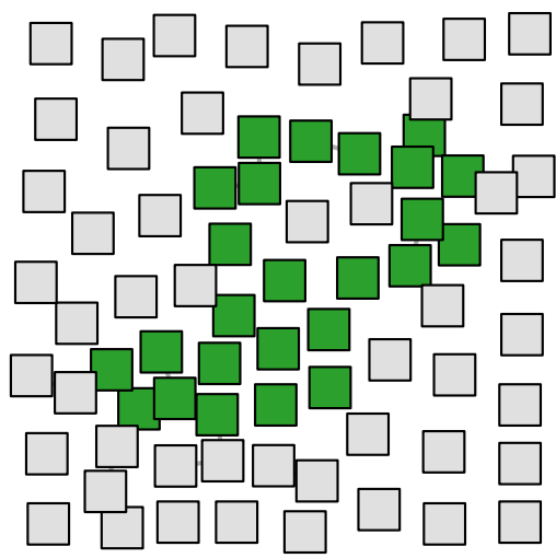
GT Label: 8
