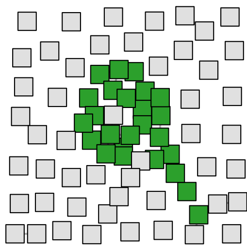
GT Label: 9
