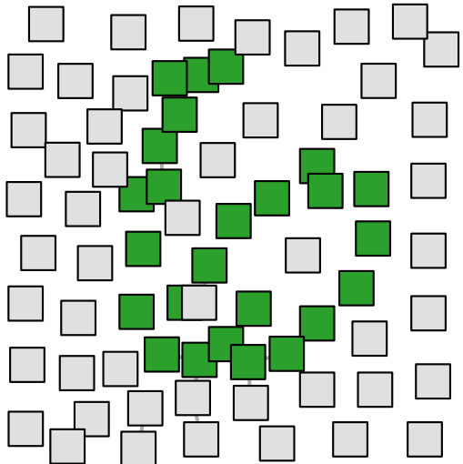
GT Label: 6
