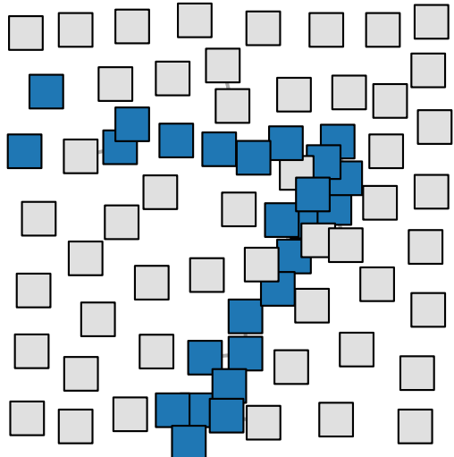
Predicted: 7
