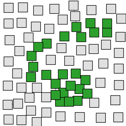
GT Label: 5
