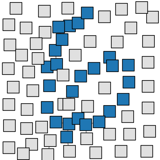
Predicted: 6
