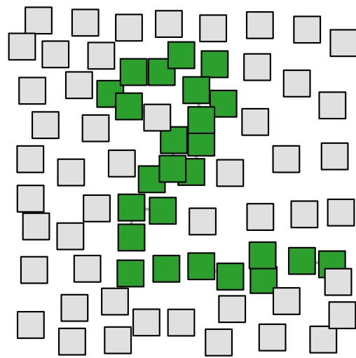
GT Label: 2
