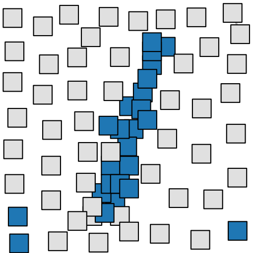
Predicted: 1
