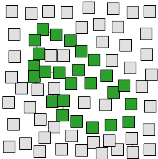
GT Label: 3
