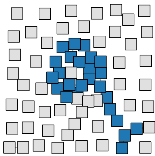
Predicted: 9
