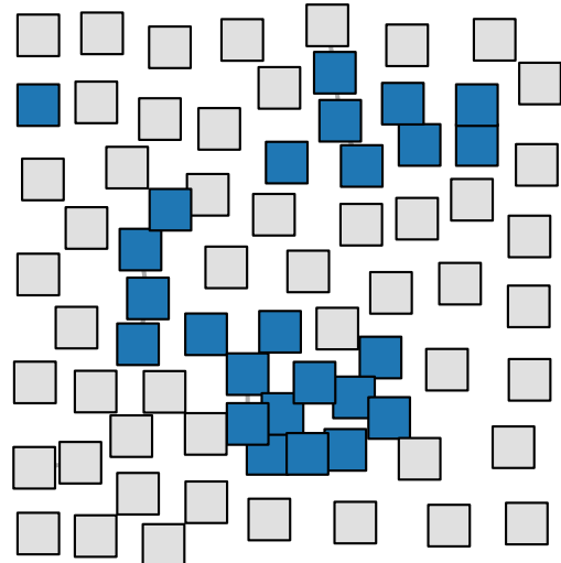
Predicted: 4
