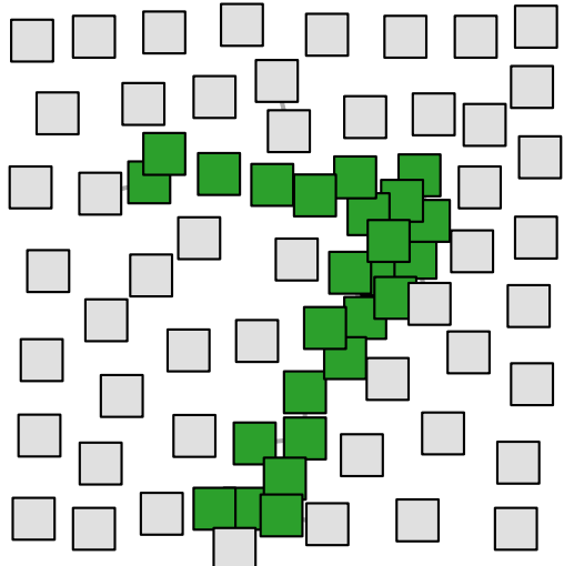
GT Label: 7
