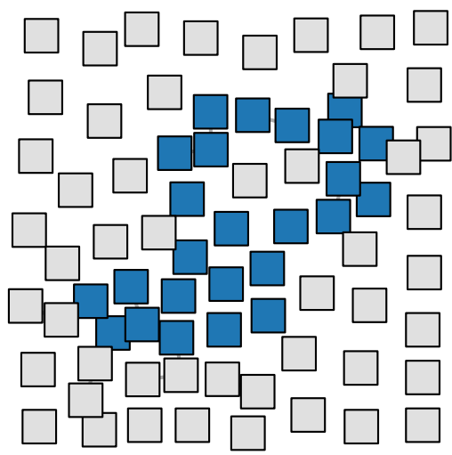
Predicted: 8
