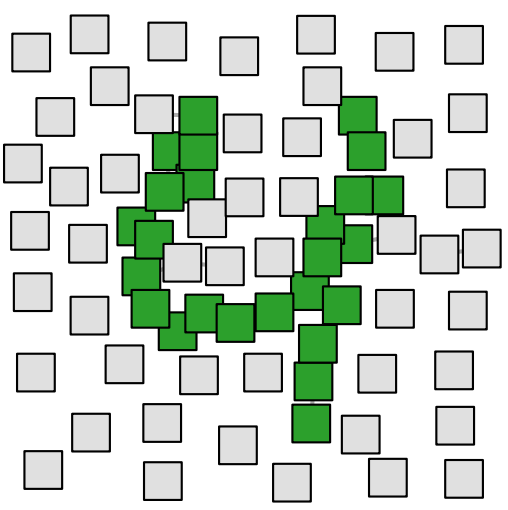
GT Label: 4
