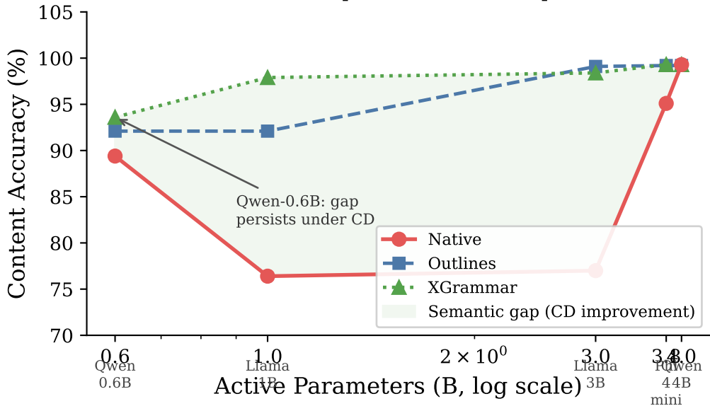
(b) Semantic: Gap Persists, Scale-Dependent
