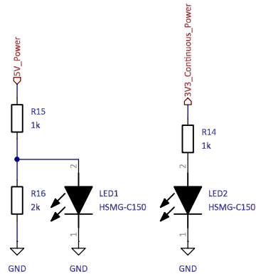
LED driver
