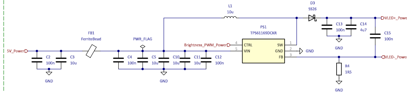
LED driver
