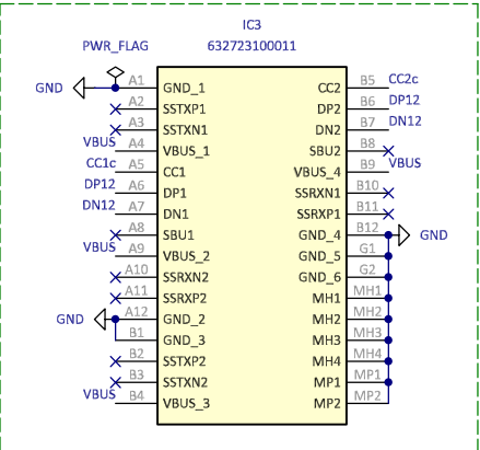
USB-C connector right angle
