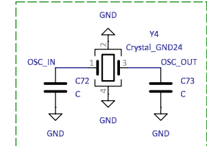
LAN8651 25MHz oscillator
