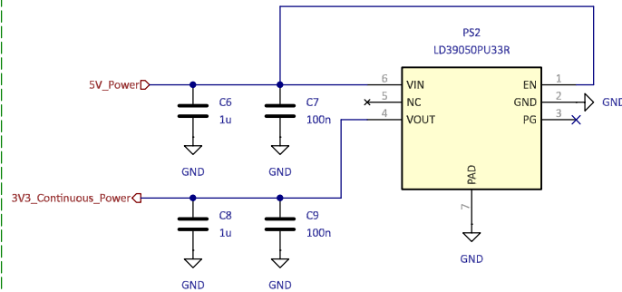
LDO 5V -> 3.3V
