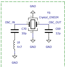
Crystal oscillator
