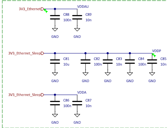
Ethernet LAN8651 decoupling capacitors
