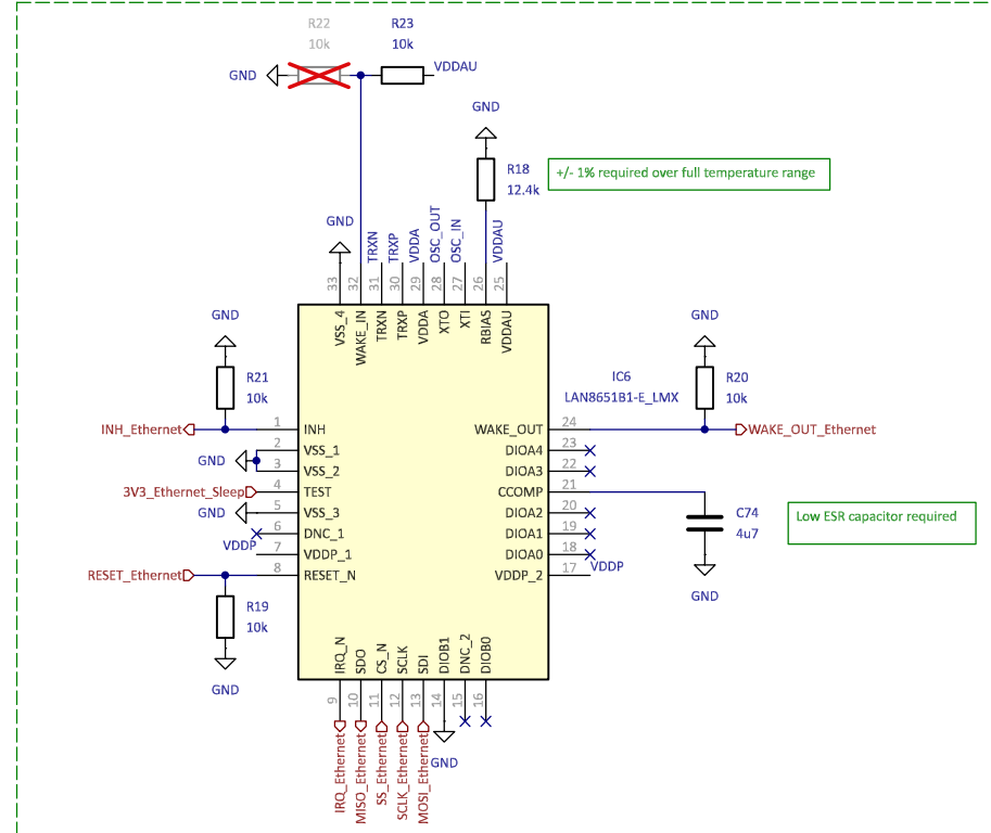
External Ethernet PHY
